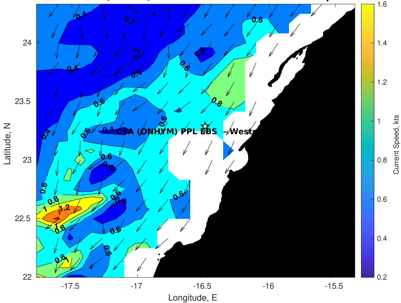
Surface Currents for CSA (ONHYM) PPL EBS - Western Sahara at 29-Apr-2025 00:00:00
