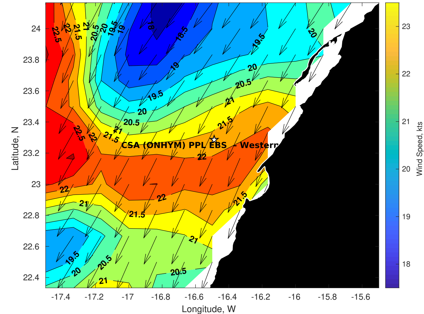
Winds (kts) for CSA (ONHYM) PPL EBS - Western Sahara at 30-Apr-2025 09:00:00
