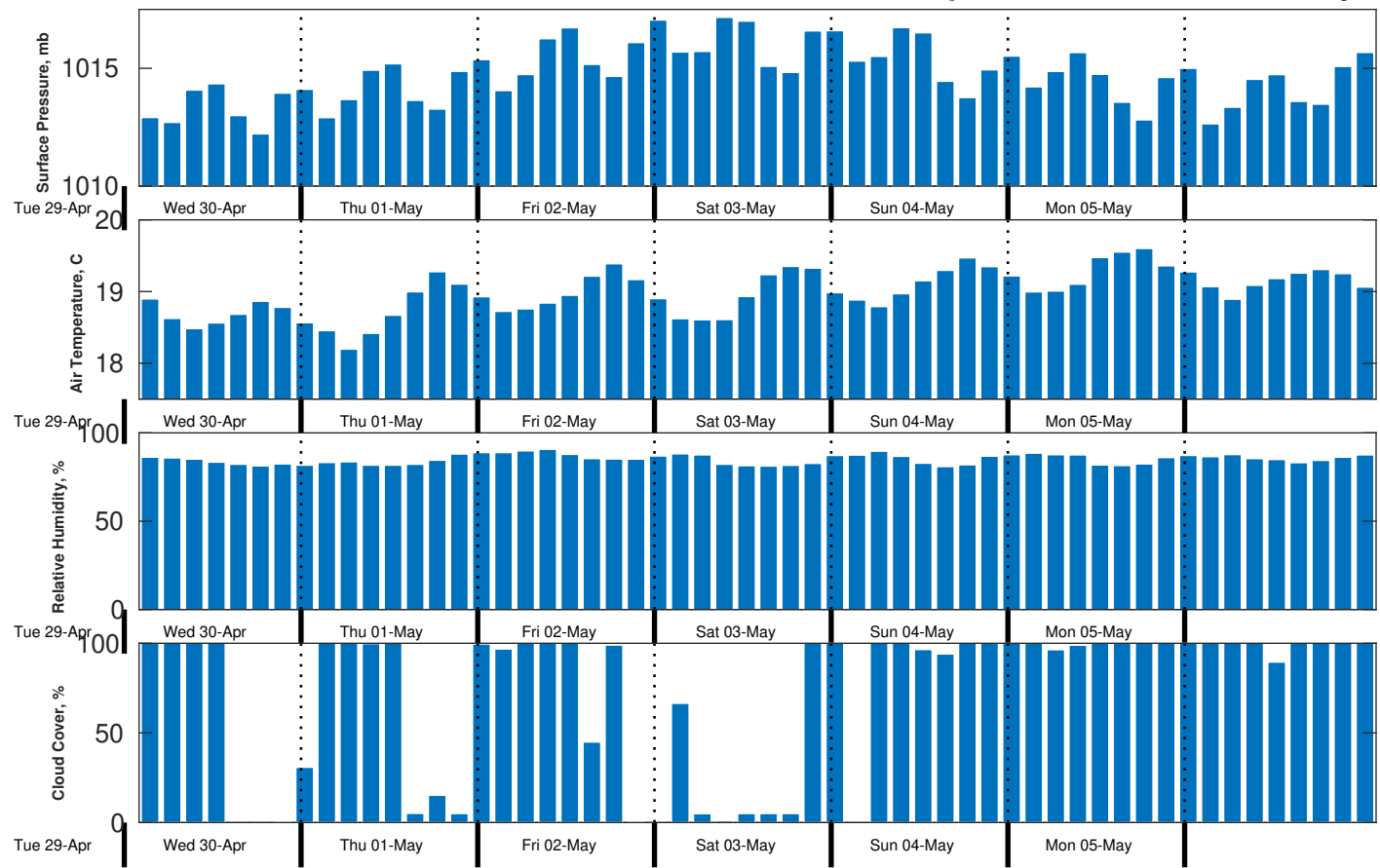
Met Forecast for CSA (ONHYM) PPL EBS - Western Sahara from 30-Apr-2025 00:00:00 to 07-May-2025 00:00:00
