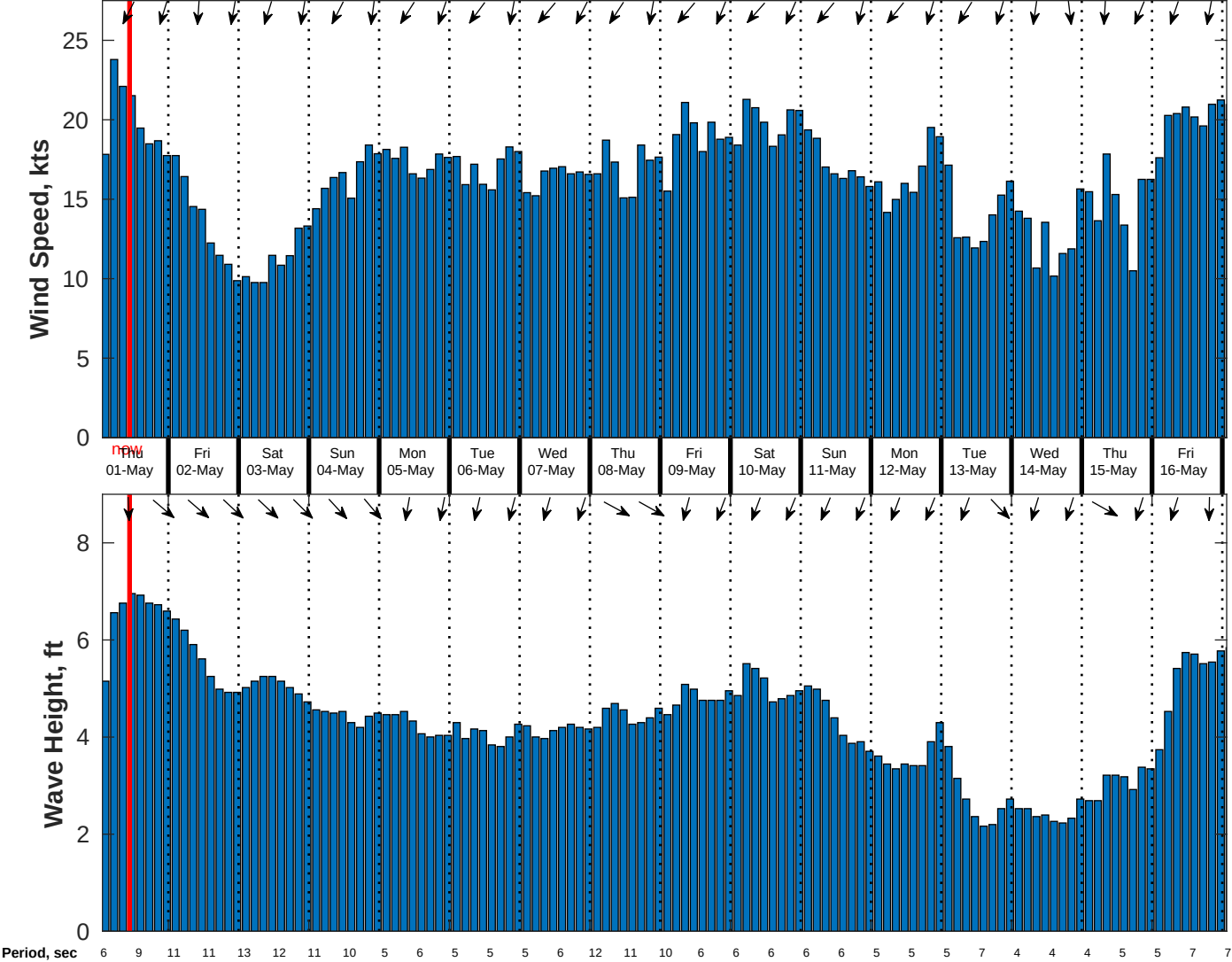
Wind & Wave Forecast for CSA (ONHYM) PPL EBS - Western Sahara from 30-Apr-2025 01:00:00 to 16-May-2025 01:00:00
