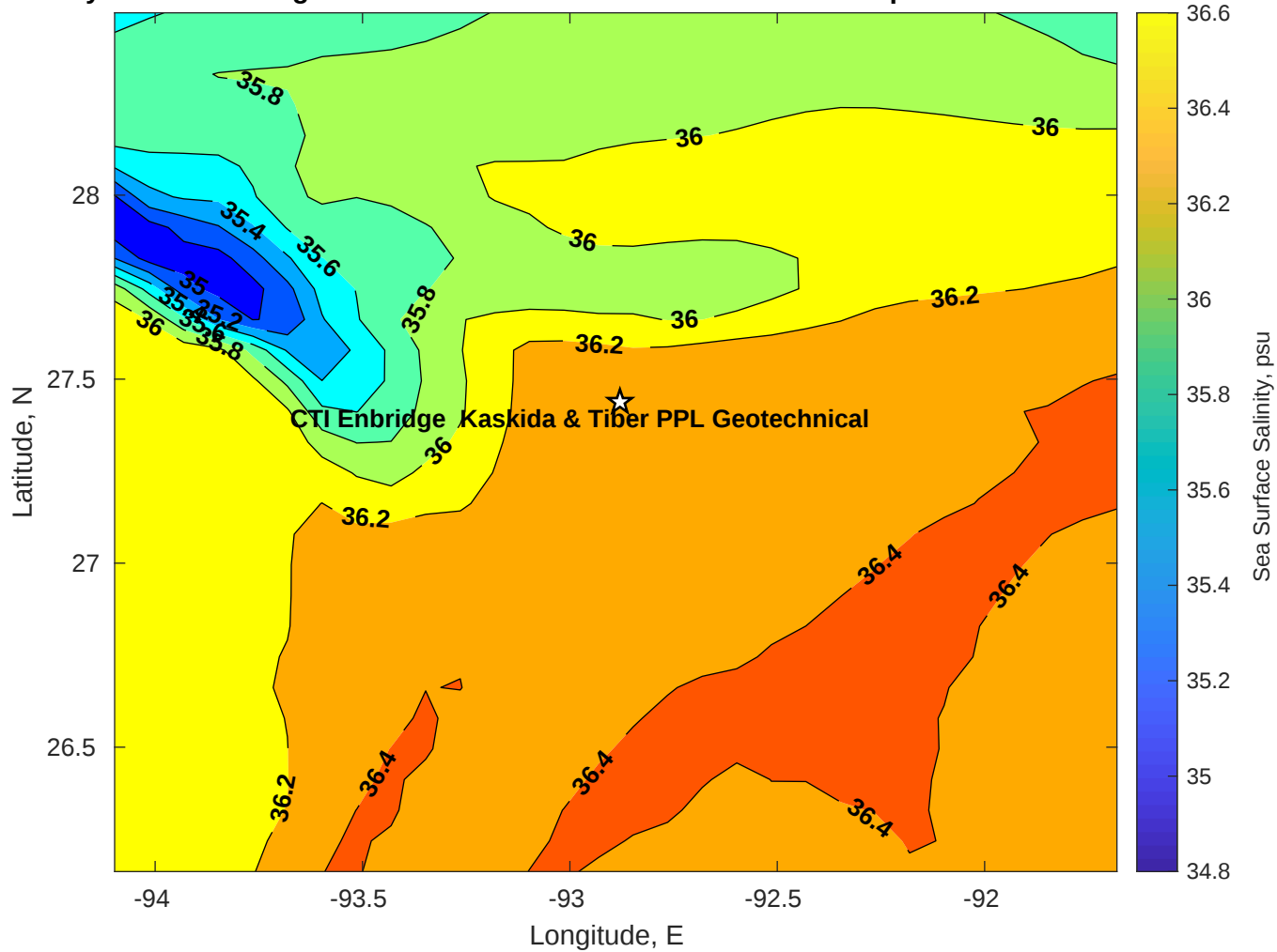
Surface Salinity for CTI Enbridge Kaskida & Tiber PPL Geotechnical at 29-Apr-2025 00:00:00
