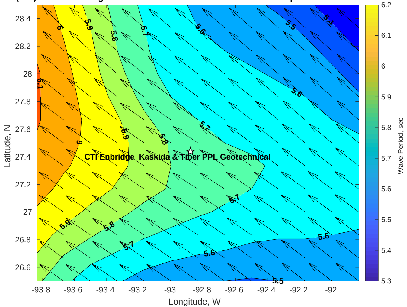
Wave Period (sec) for CTI Enbridge Kaskida & Tiber PPL Geotechnical at 30-Apr-2025 09:00:00
