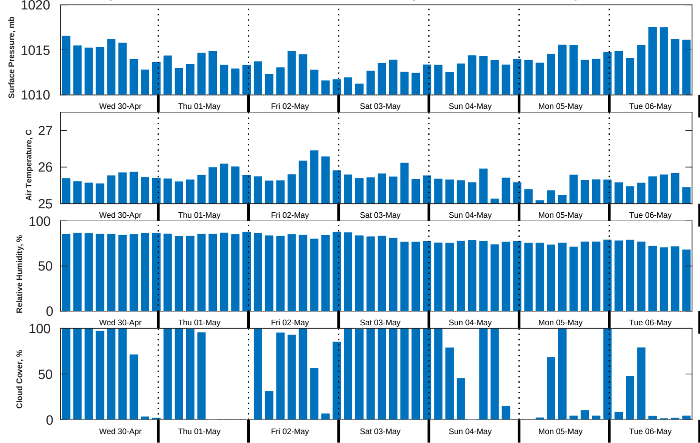
Met Forecast for CTI Enbridge Kaskida & Tiber PPL Geotechnical from 30-Apr-2025 00:00:00 to 07-May-2025 00:00:00
