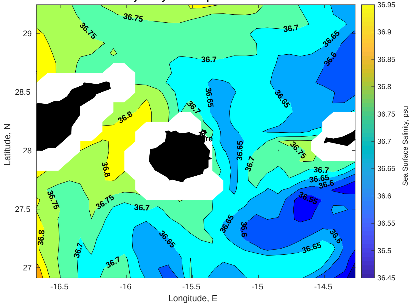
Surface Salinity for Gyre at 29-Apr-2025 00:00:00
