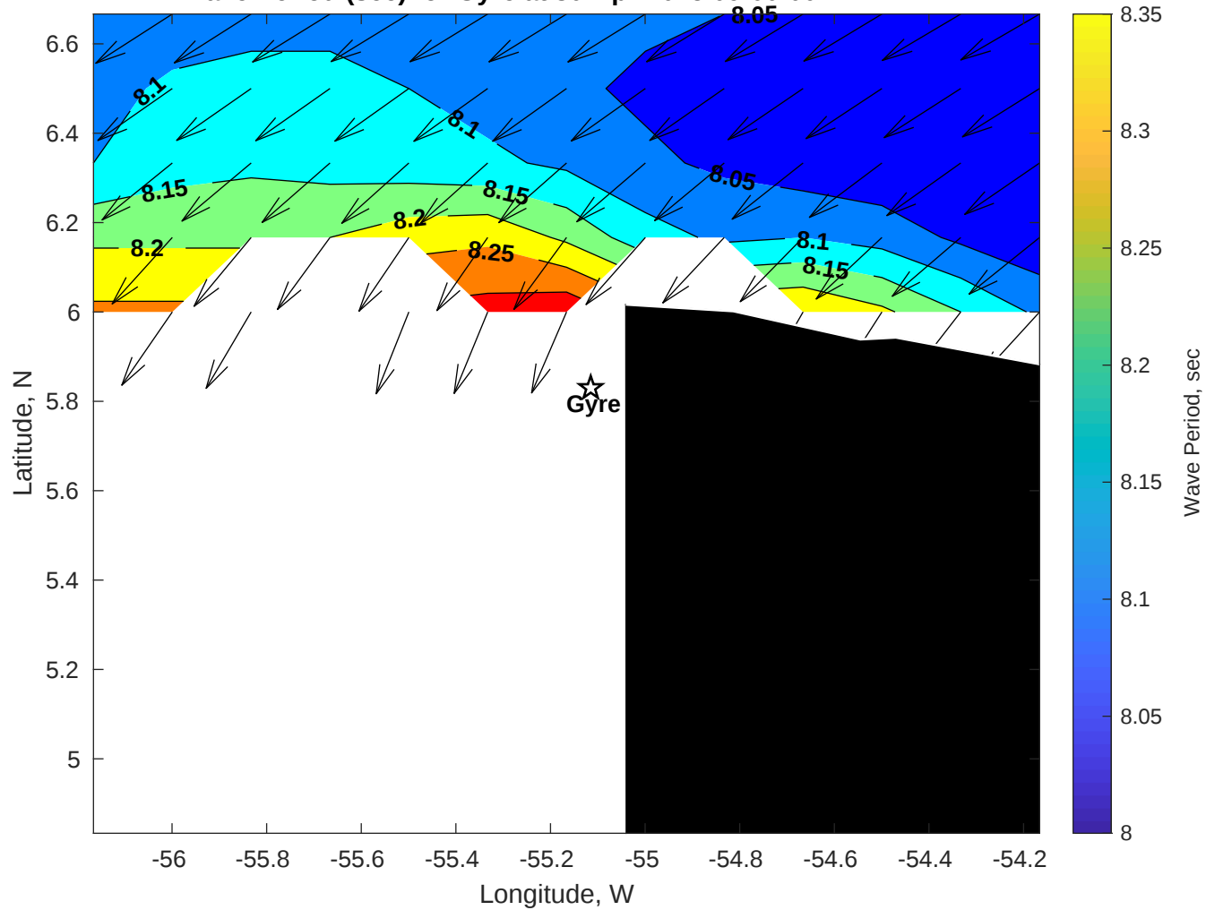
Wave Period (sec) for Gyre at 30-Apr-2025 09:00:00
