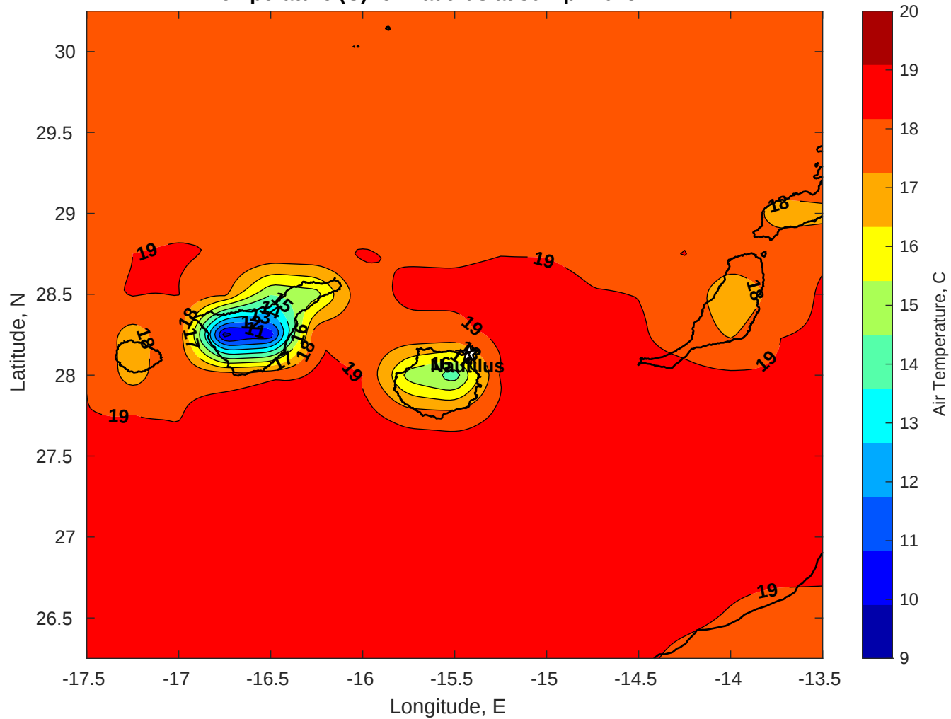
Air Temperature (C) for Nautilus at 30-Apr-2025
