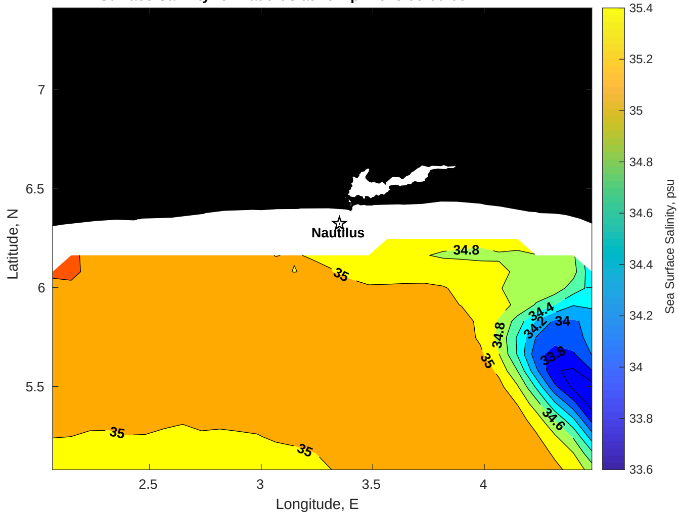
Surface Salinity for Nautilus at 29-Apr-2025 00:00:00
