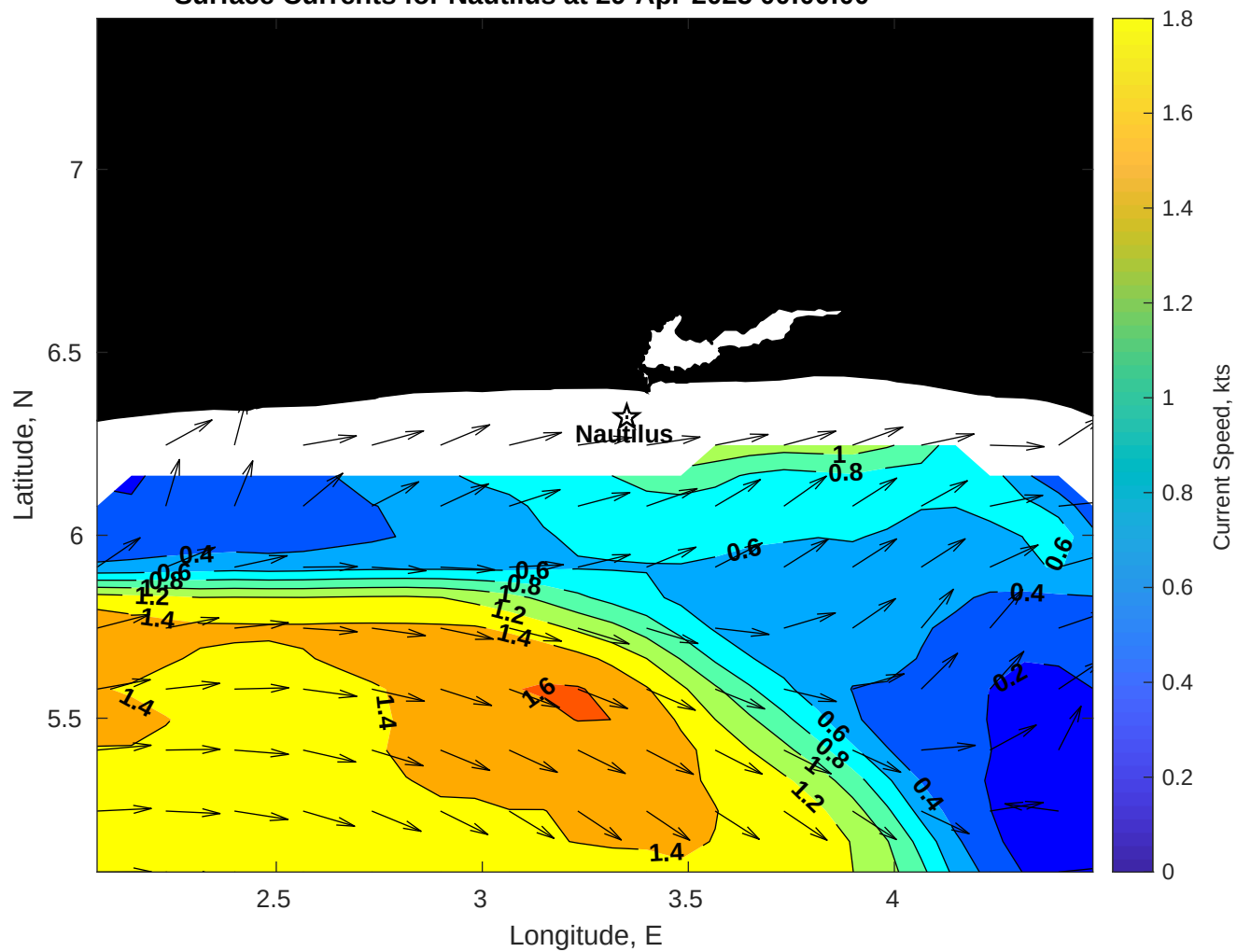
Surface Currents for Nautilus at 29-Apr-2025 00:00:00
