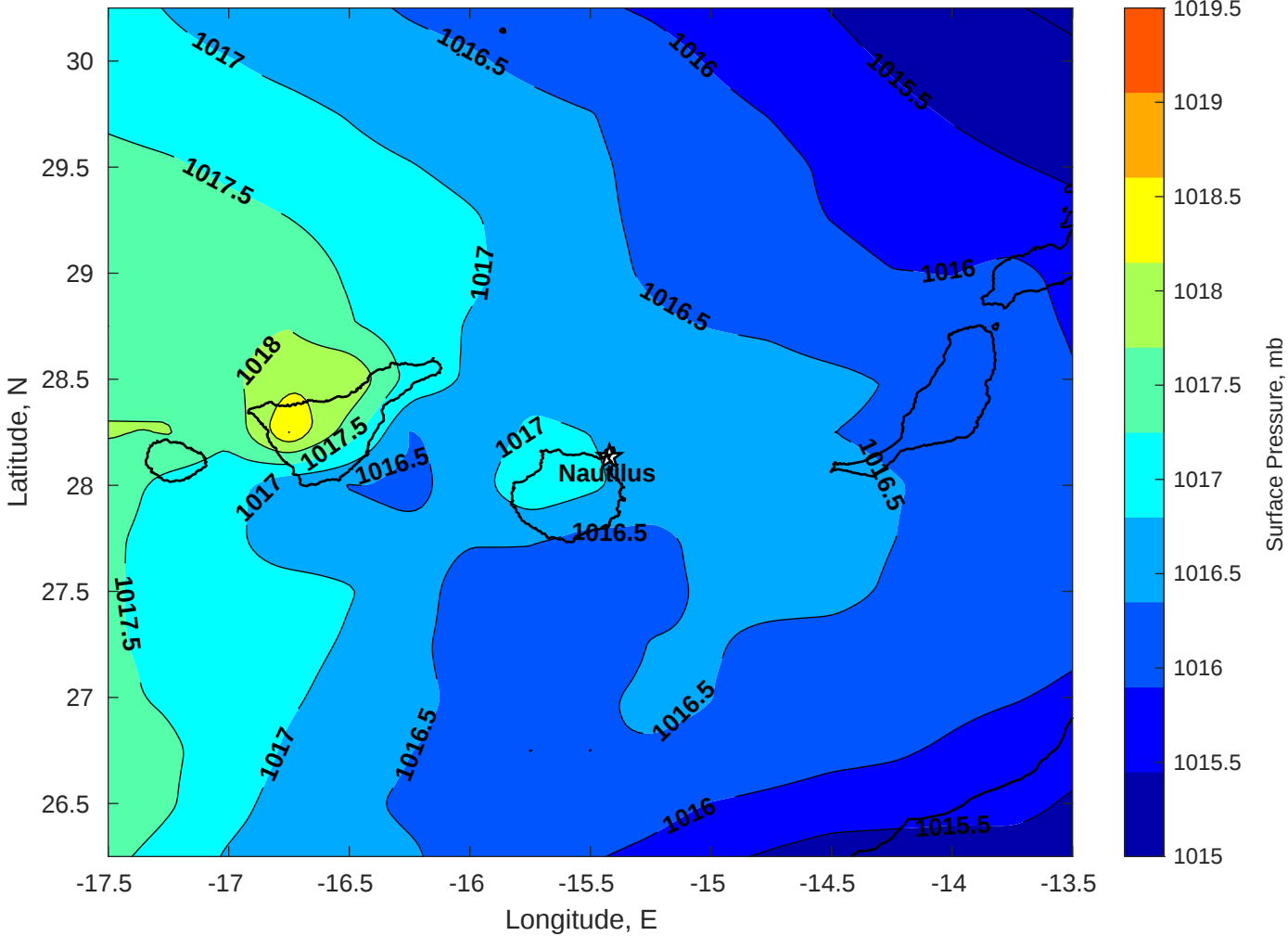
Surface Pressure (mb) for Nautilus at 30-Apr-2025 00:00:00
