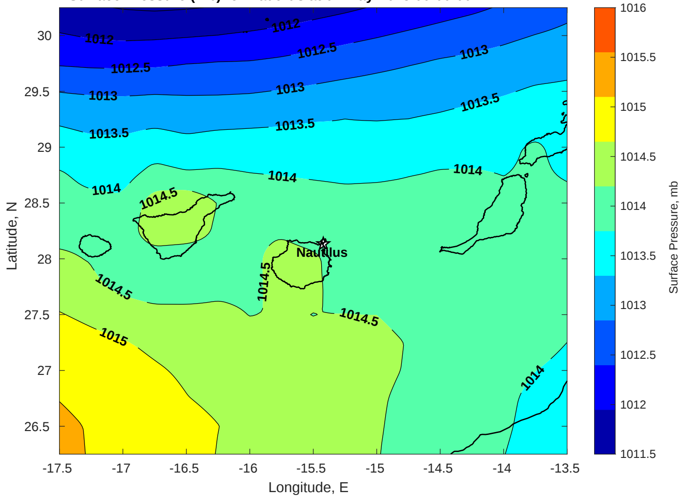
Surface Pressure (mb) for Nautilus at 01-May-2025 00:00:00
