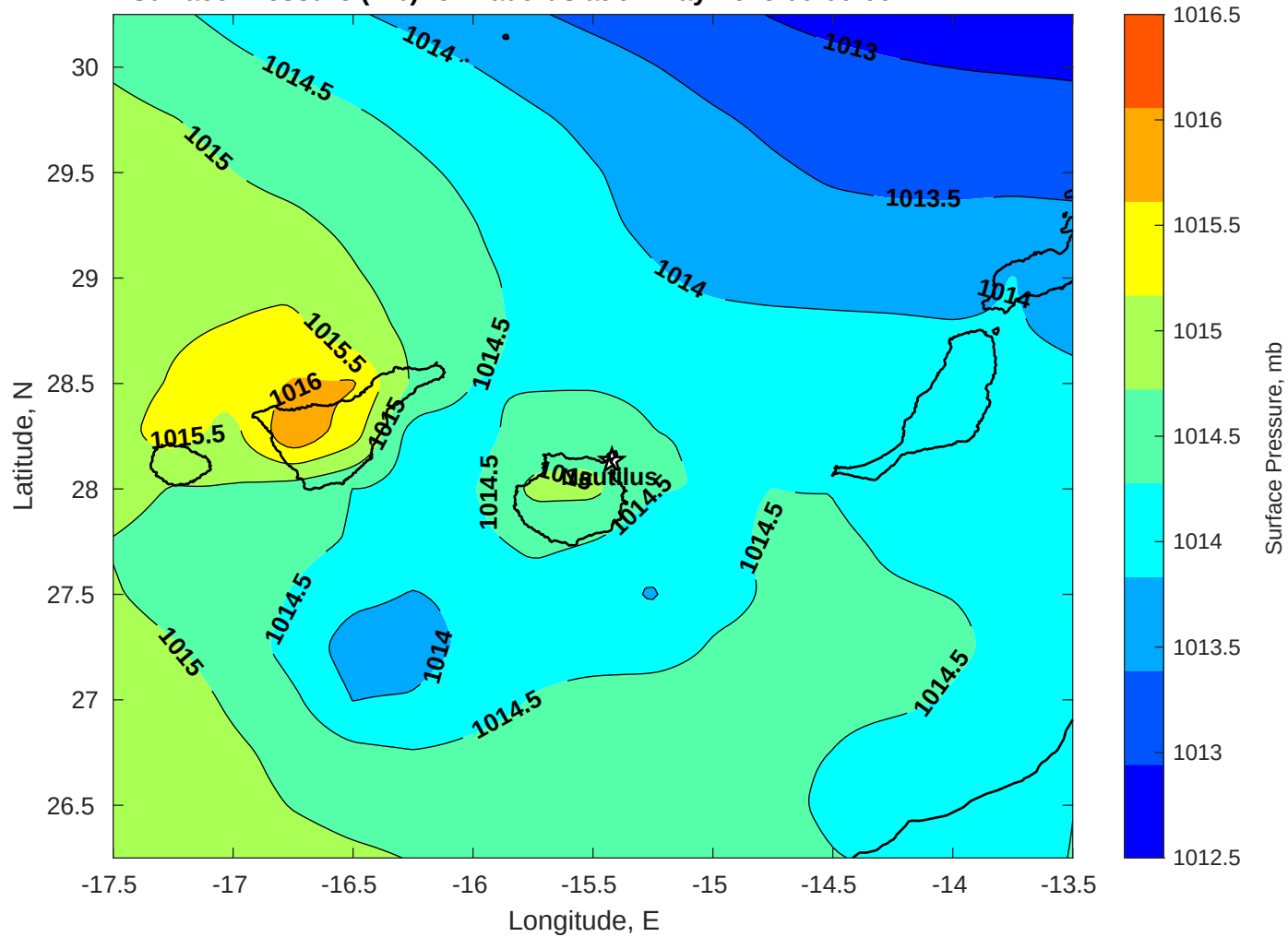
Surface Pressure (mb) for Nautilus at 02-May-2025 00:00:00
