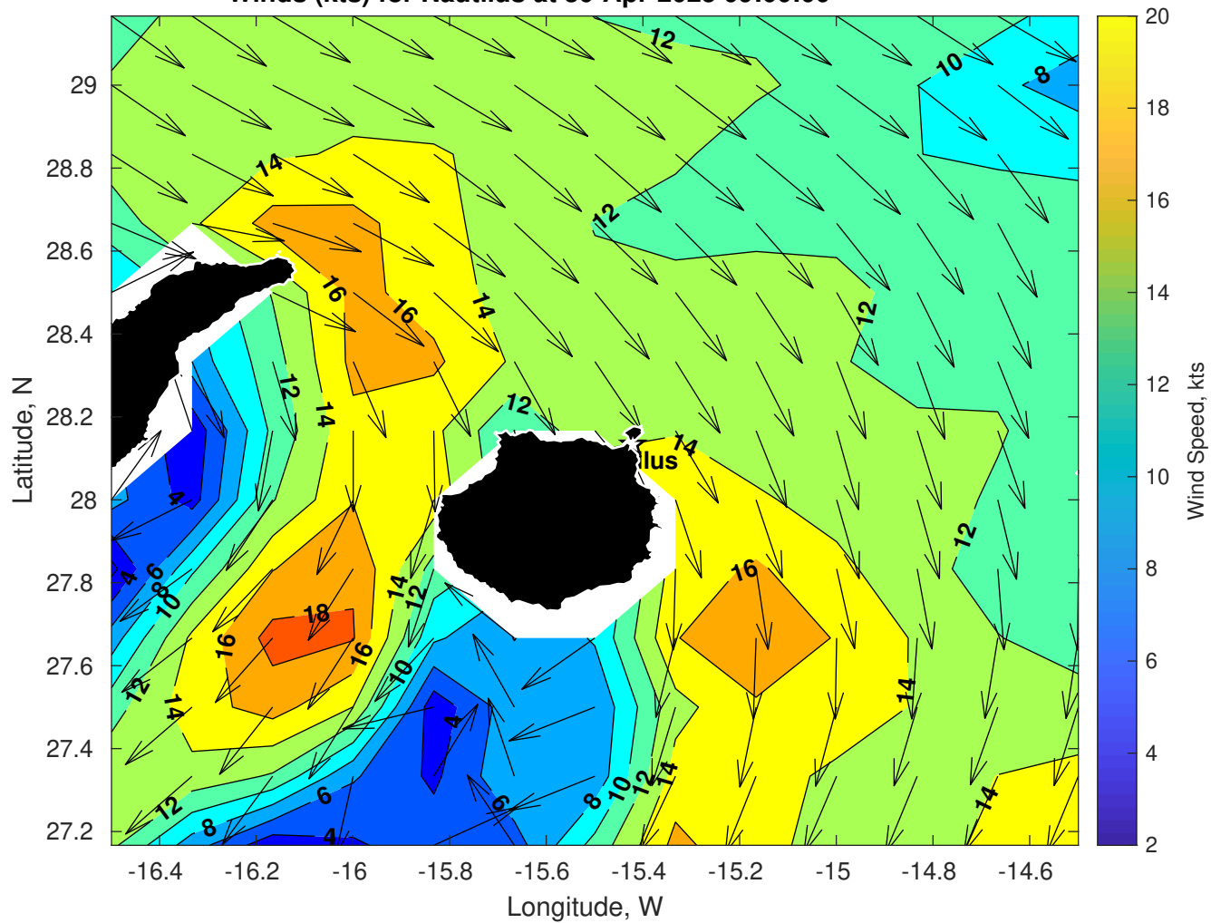
Winds (kts) for Nautilus at 30-Apr-2025 09:00:00
