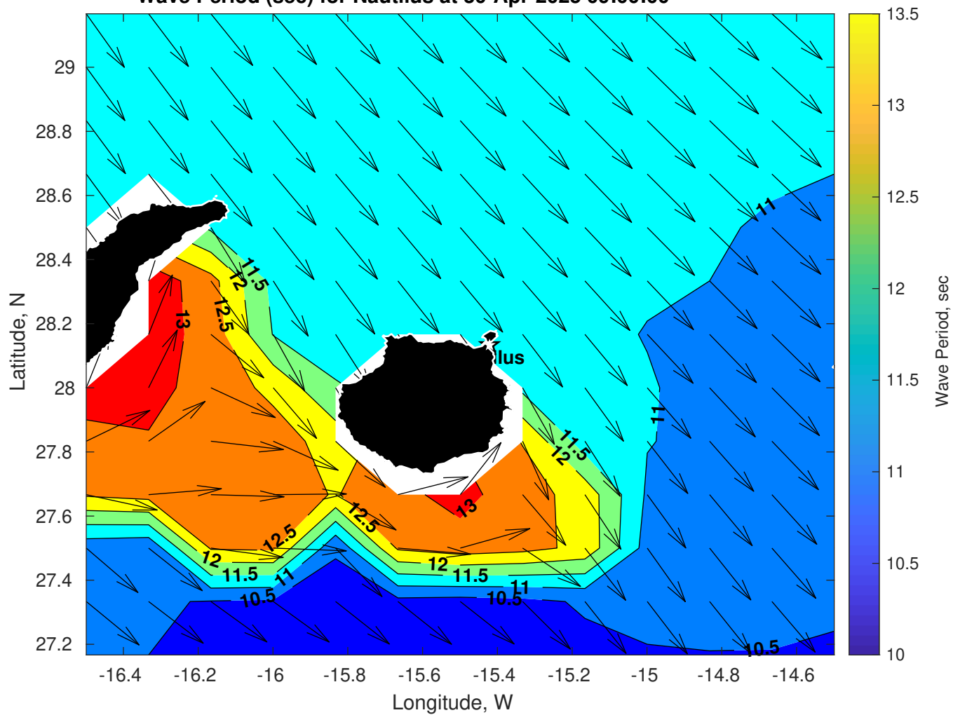
Wave Period (sec) for Nautilus at 30-Apr-2025 09:00:00
