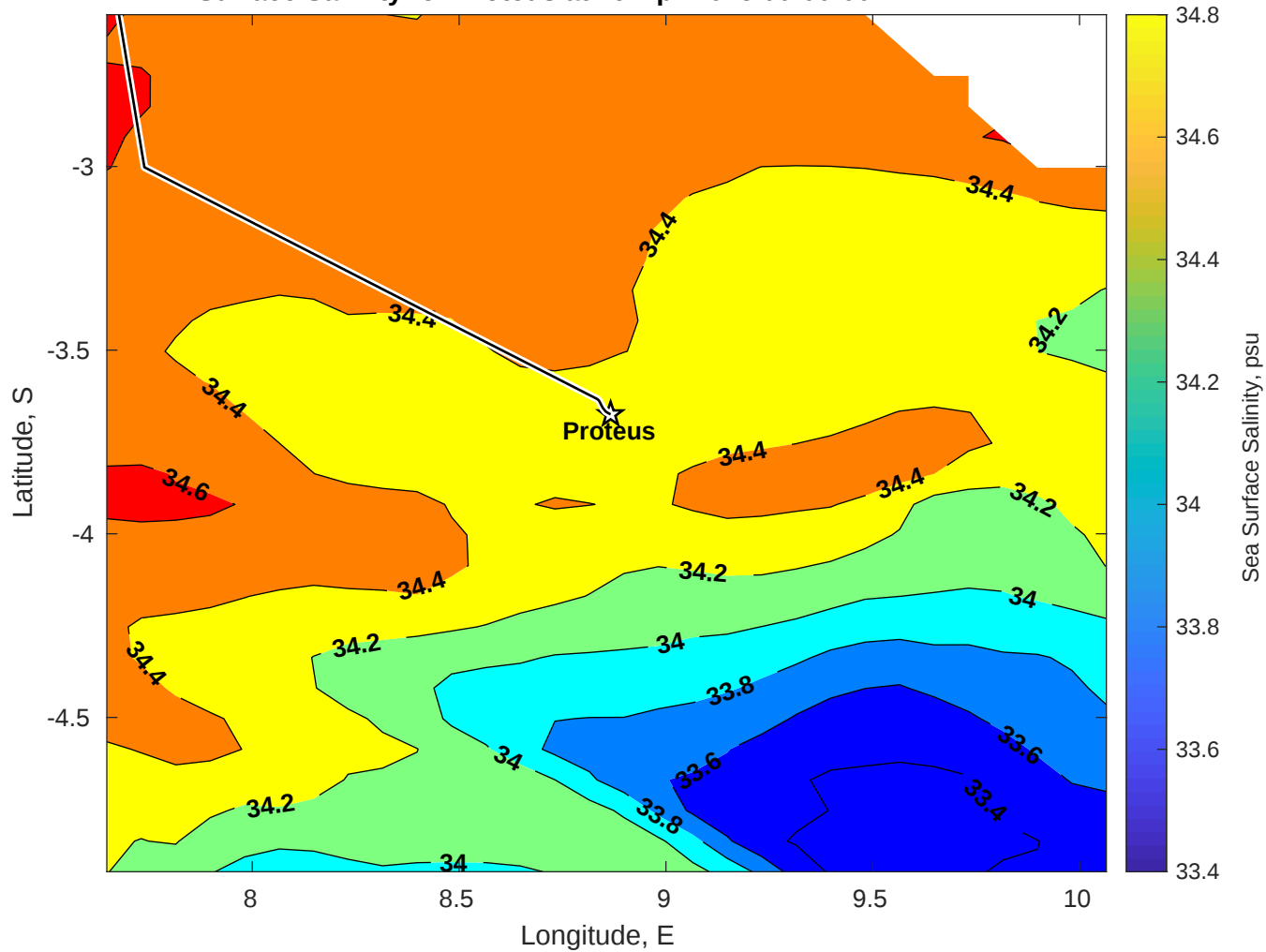
Surface Salinity for Proteus at 29-Apr-2025 00:00:00
