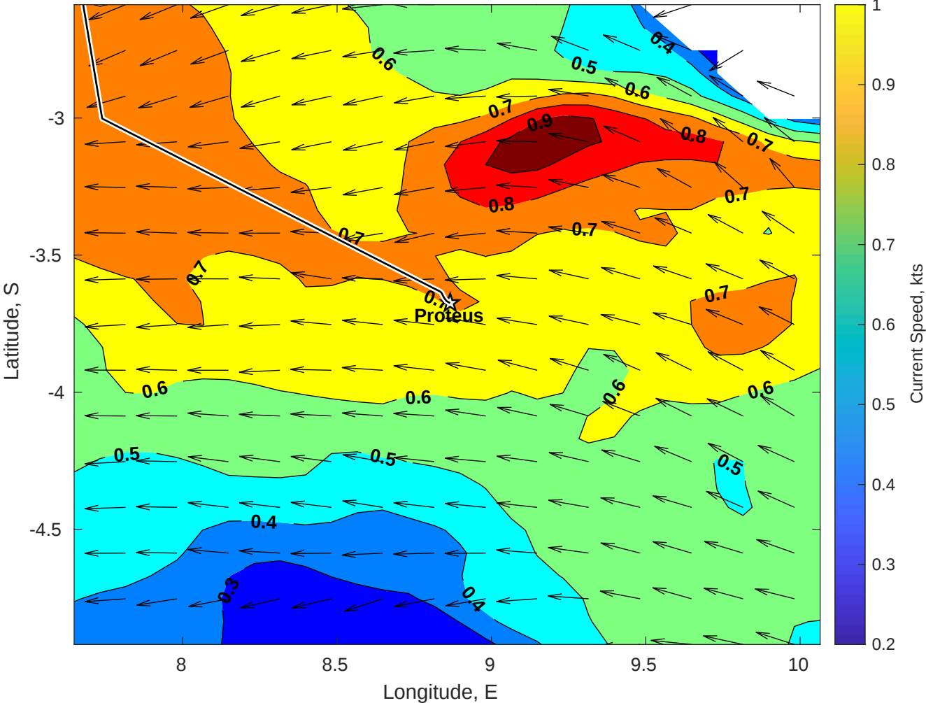
Surface Currents for Proteus at 29-Apr-2025 00:00:00
