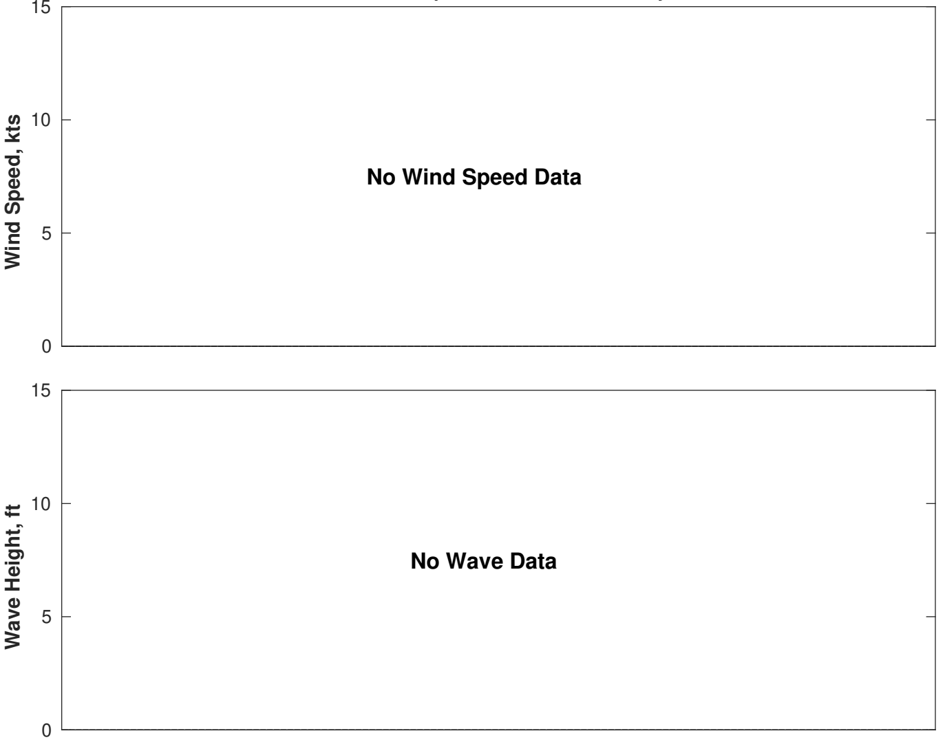
Wind & Wave Forecast for Proteus from 30-Apr-2025 01:00:00 to 16-May-2025 01:00:00
