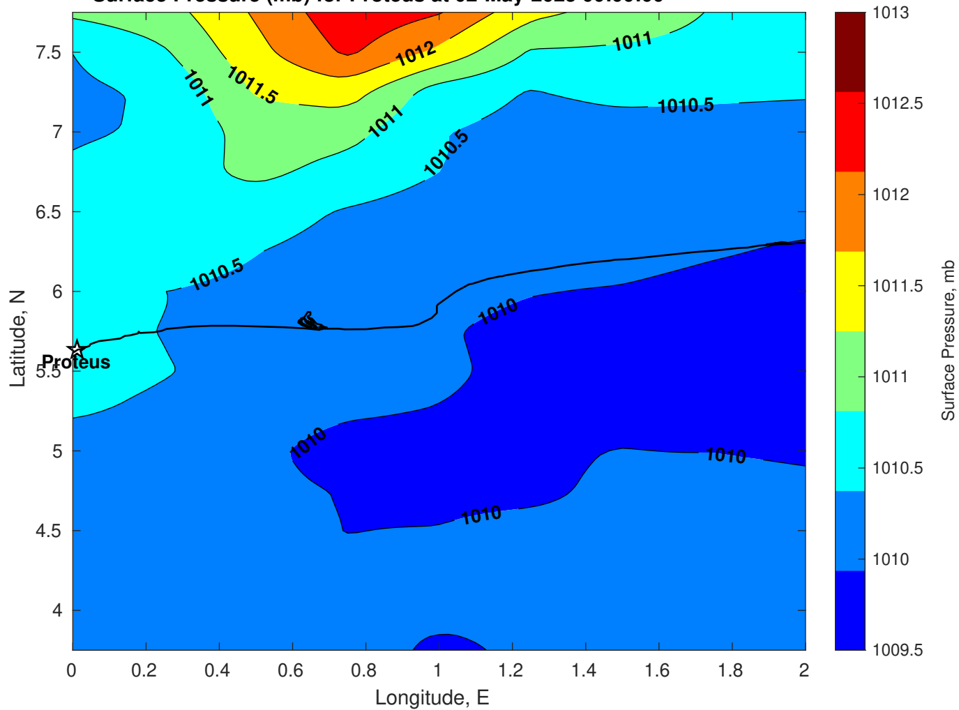
Surface Pressure (mb) for Proteus at 02-May-2025 00:00:00
