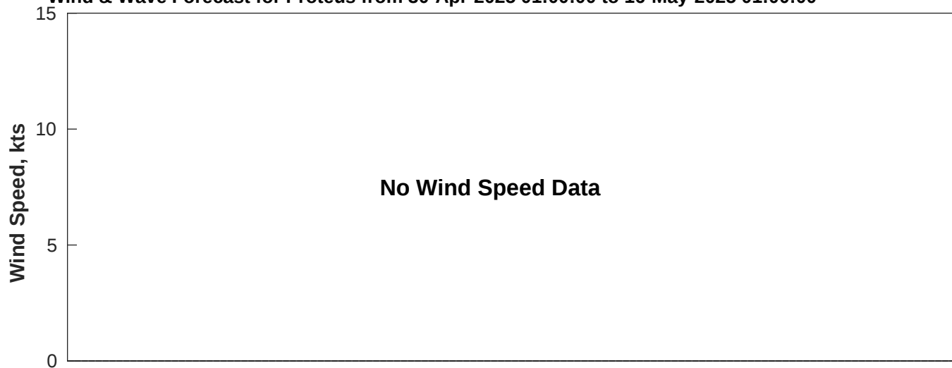
Wind & Wave Forecast for Proteus from 30-Apr-2025 01:00:00 to 16-May-2025 01:00:00
