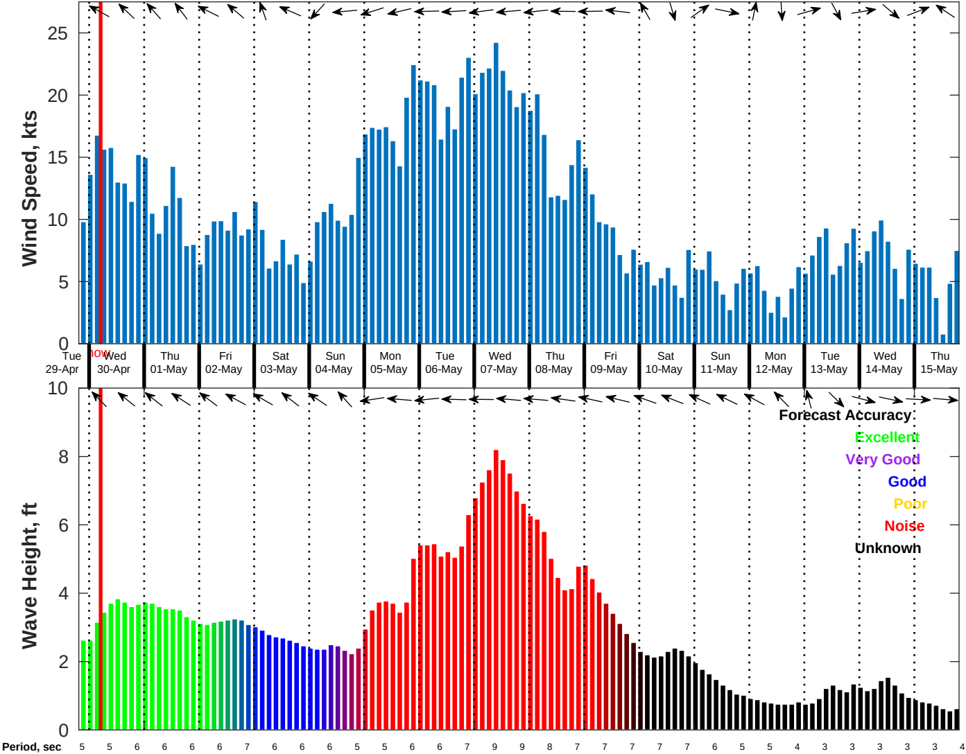
Wind & Wave Forecast for Shell Noches GC19 PPL Geotechnical from 29-Apr-2025 20:00:00 to 15-May-2025 20:00:00
