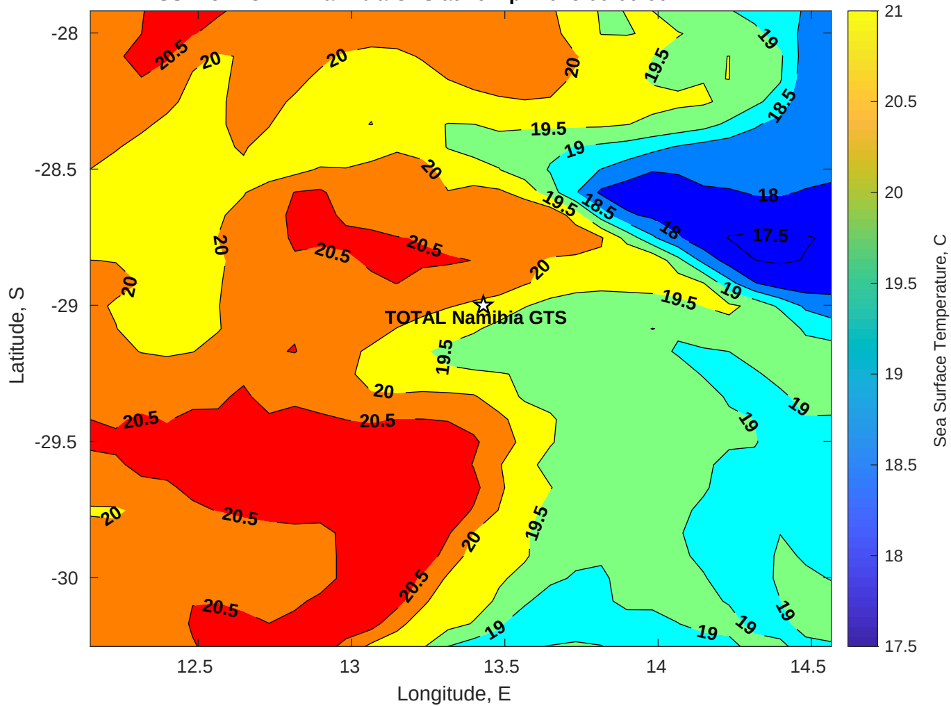
SST for TOTAL Namibia GTS at 29-Apr-2025 00:00:00
