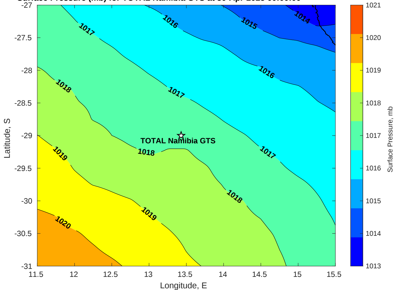
Surface Pressure (mb) for TOTAL Namibia GTS at 30-Apr-2025 00:00:00
