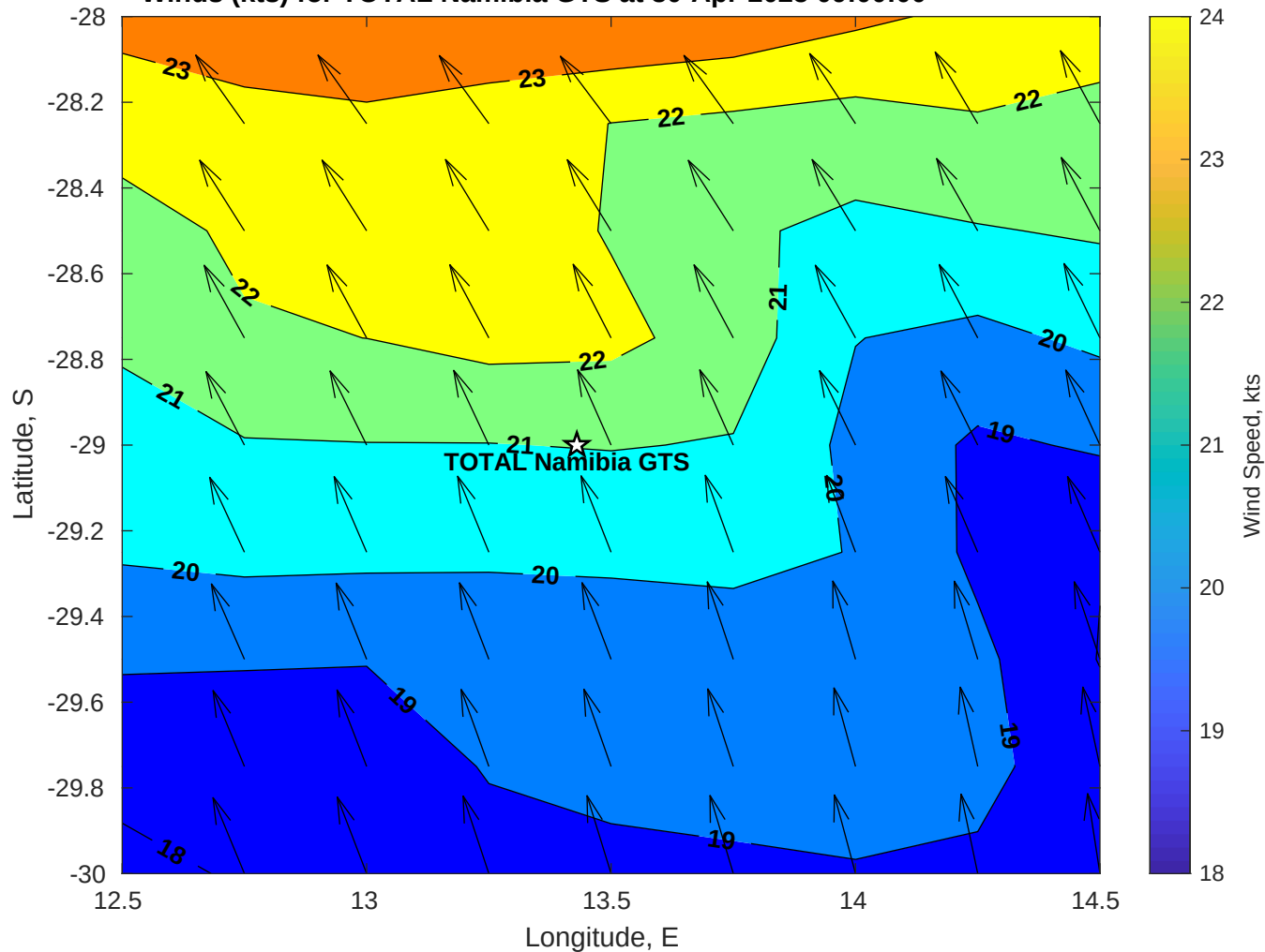
Winds (kts) for TOTAL Namibia GTS at 30-Apr-2025 09:00:00
