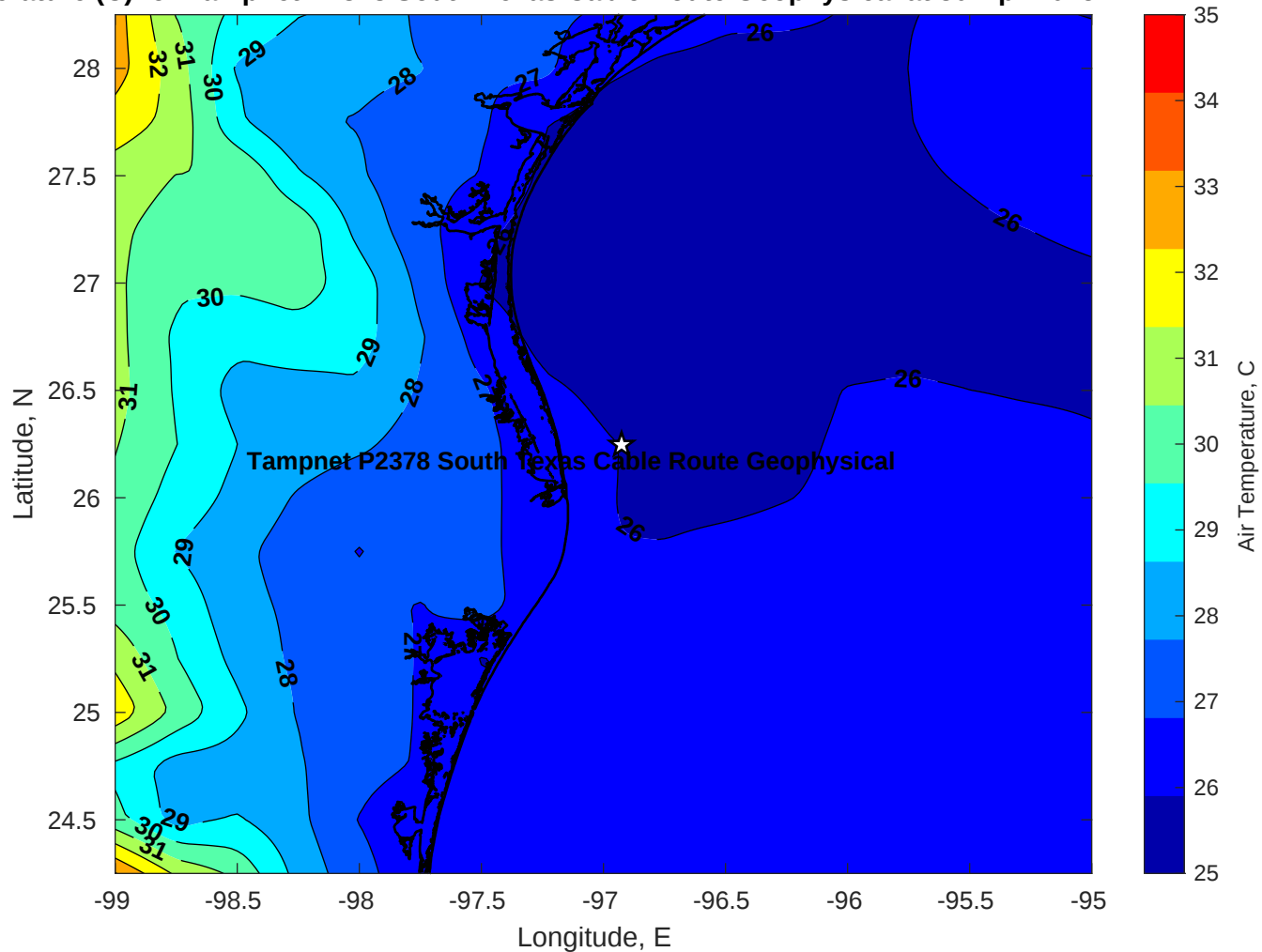
Air Temperature (C) for Tampnet P2378 South Texas Cable Route Geophysical at 30-Apr-2025
