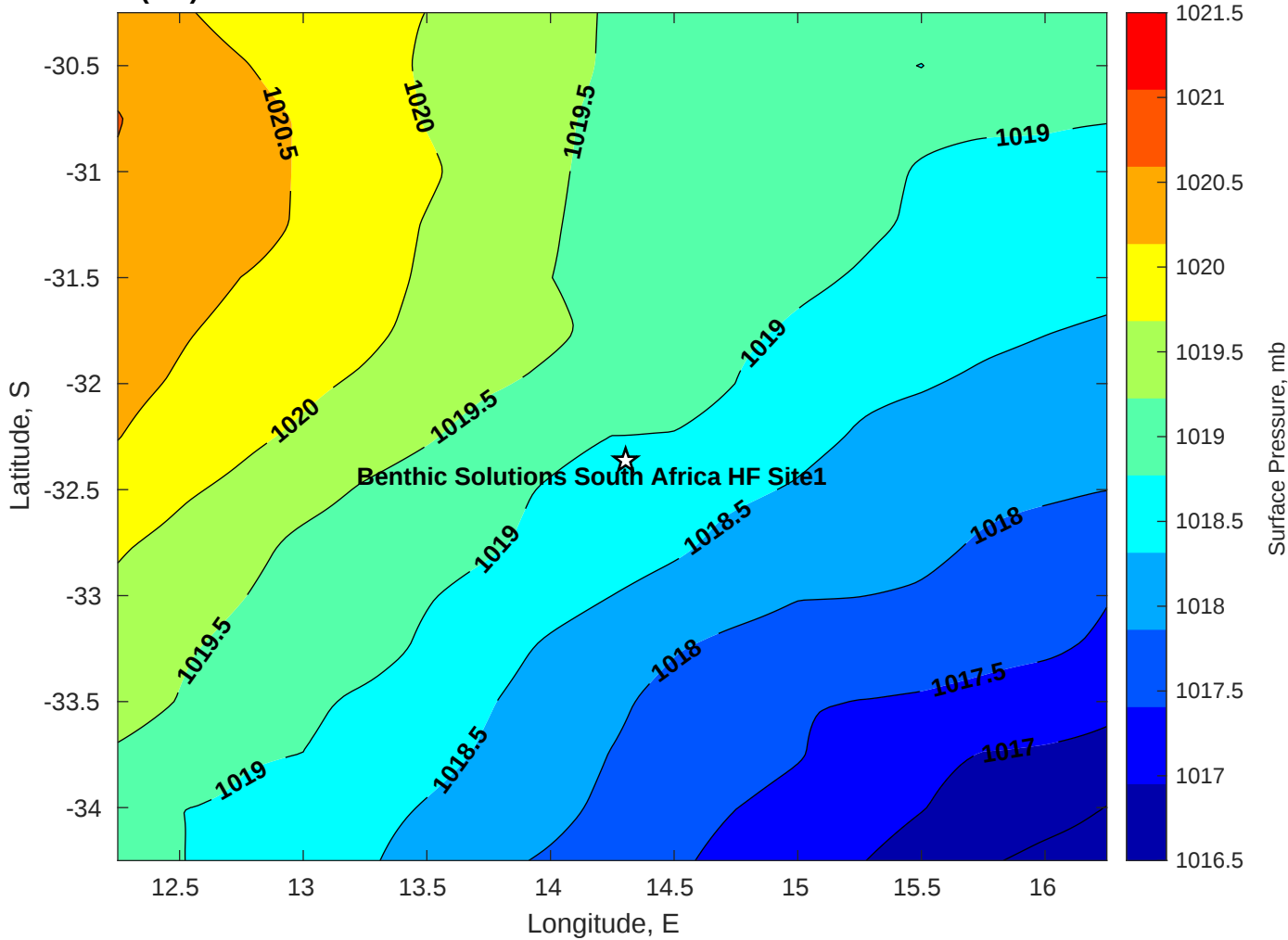
Surface Pressure (mb) for Benthic Solutions South Africa HF Site1 at 15-Nov-2030 00:00:00
