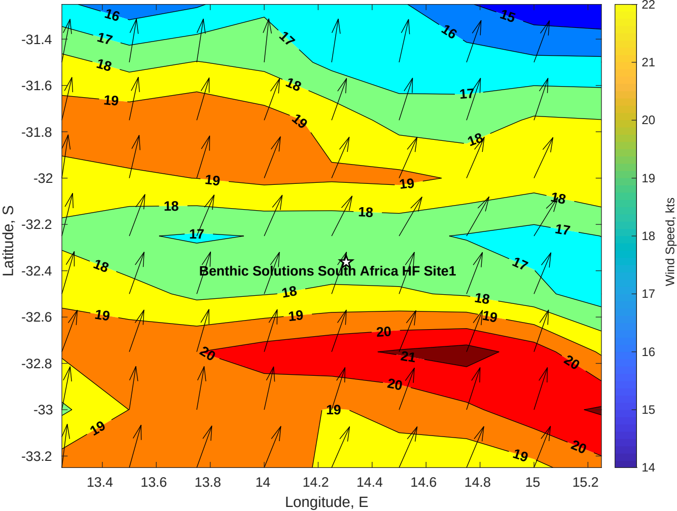
Winds (kts) for Benthic Solutions South Africa HF Site1 at 01-May-2025 09:00:00
