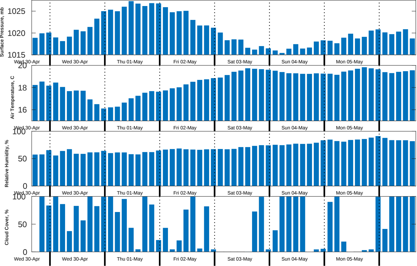
Met Forecast for Benthic Solutions South Africa HF Site1 from 30-Apr-2025 12:00:00 to 07-May-2025 12:00:00
