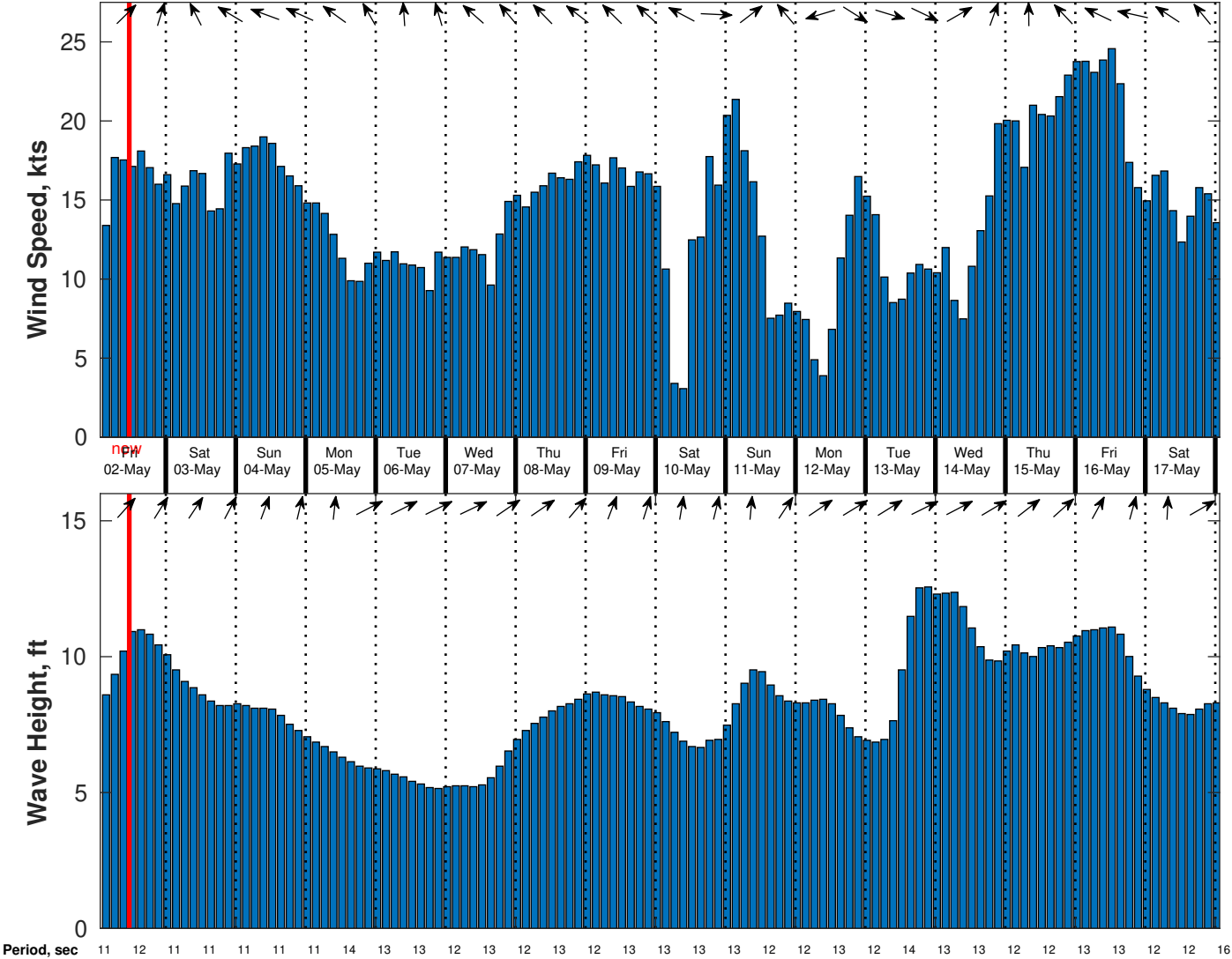
Wind & Wave Forecast for Benthic Solutions South Africa HF Site1 from 01-May-2025 02:00:00 to 17-May-2025 02:00:00
