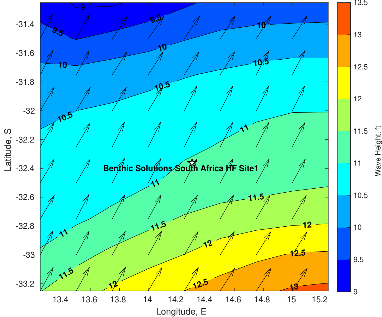
Wave Height (ft) for Benthic Solutions South Africa HF Site1 at 01-May-2025 09:00:00
