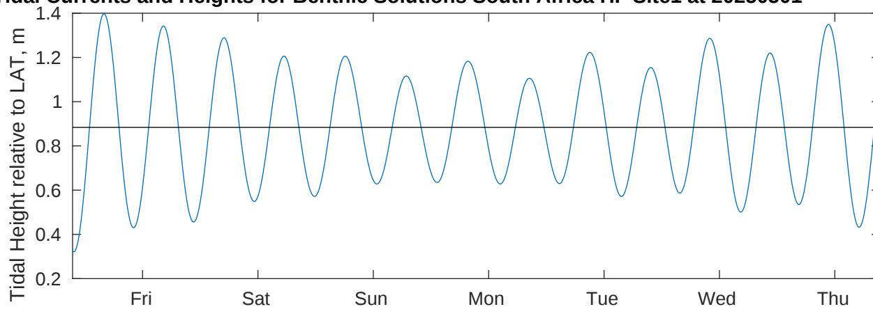
Tidal Currents and Heights for Benthic Solutions South Africa HF Site1 at 20250501
