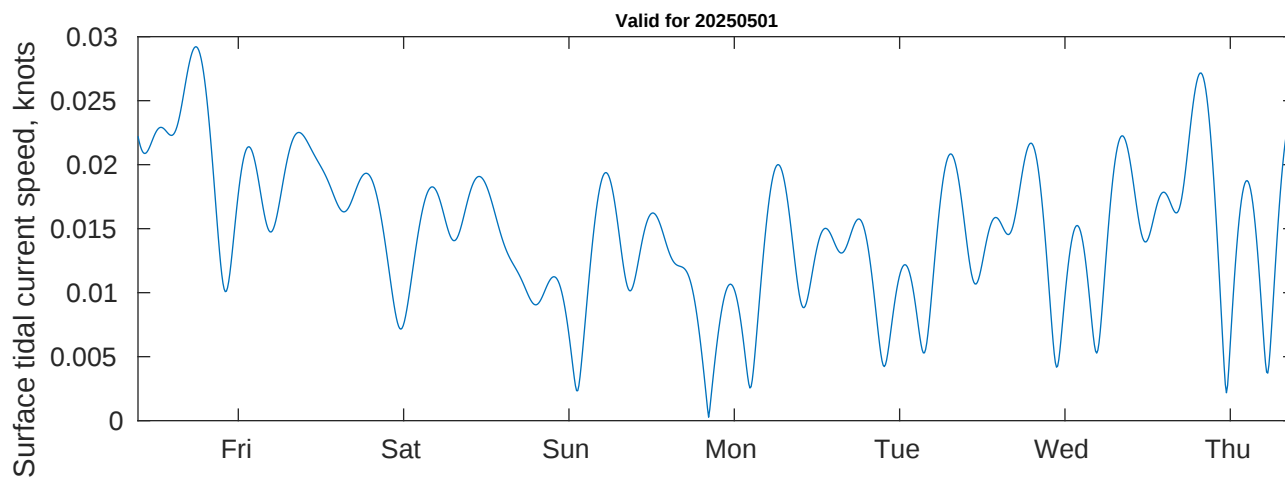
Tidal Currents and Heights for Benthic Solutions South Africa HF Site1 at 20250501
