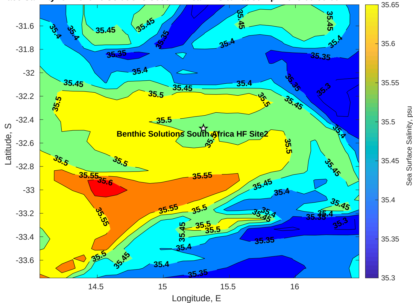
Surface Salinity for Benthic Solutions South Africa HF Site2 at 30-Apr-2025 00:00:00
