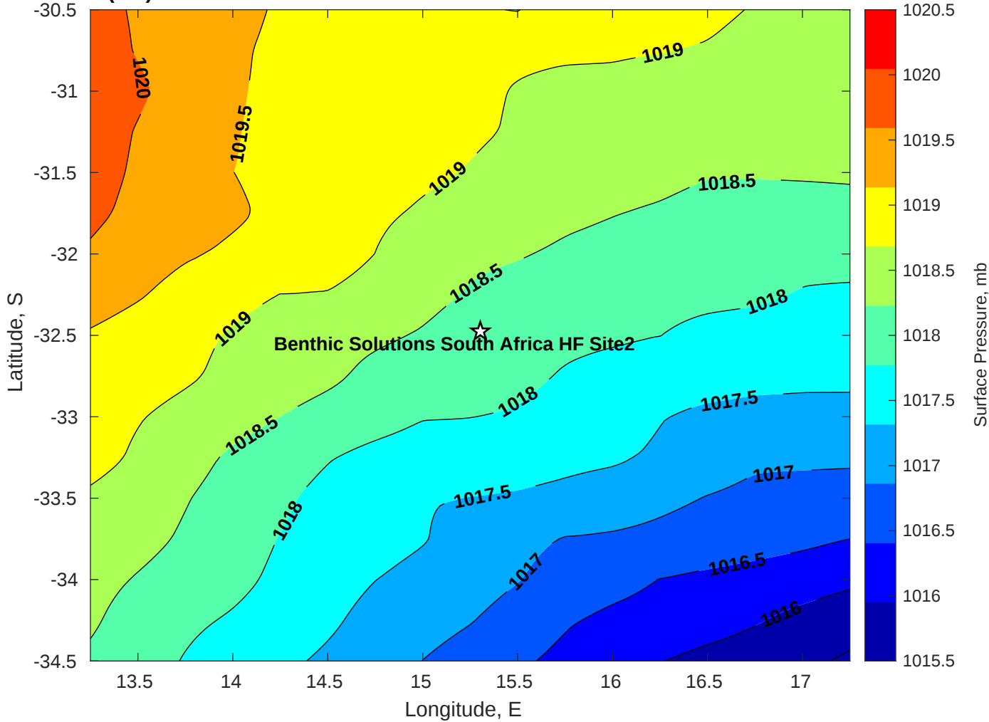
Surface Pressure (mb) for Benthic Solutions South Africa HF Site2 at 15-Nov-2030 00:00:00
