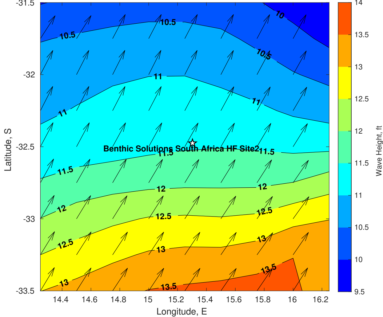
Wave Height (ft) for Benthic Solutions South Africa HF Site2 at 01-May-2025 09:00:00
