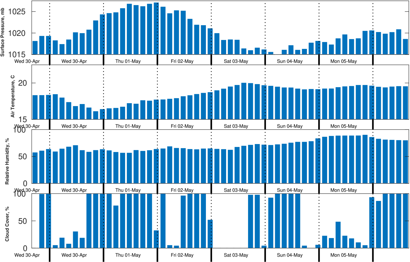
Met Forecast for Benthic Solutions South Africa HF Site2 from 30-Apr-2025 12:00:00 to 07-May-2025 12:00:00
