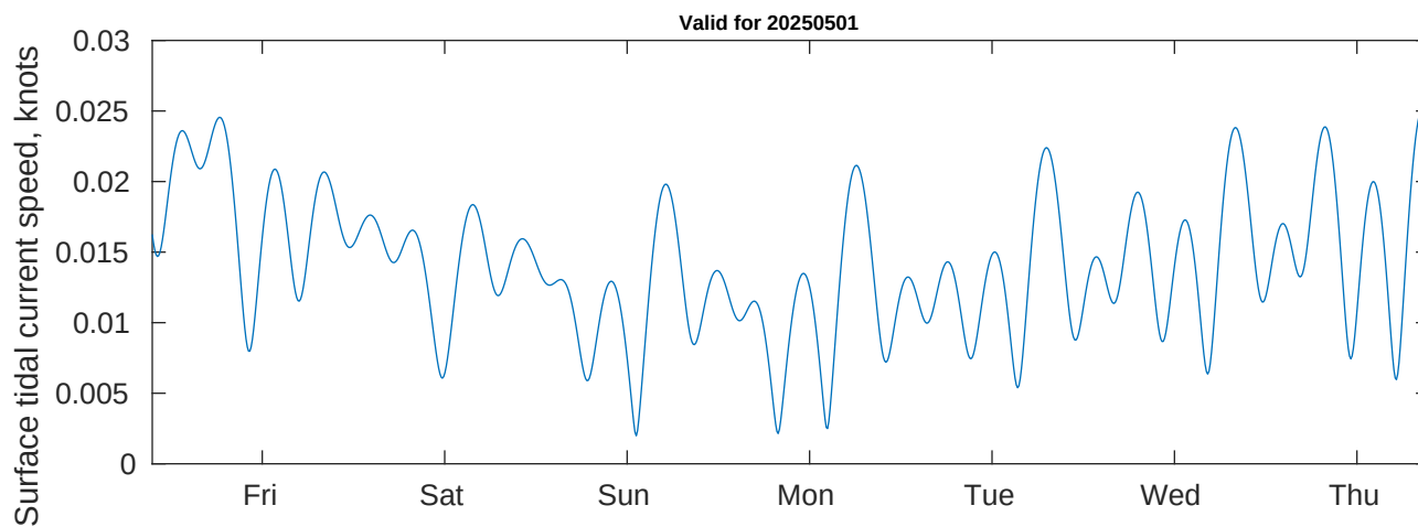
Tidal Currents and Heights for Benthic Solutions South Africa HF Site2 at 20250501
