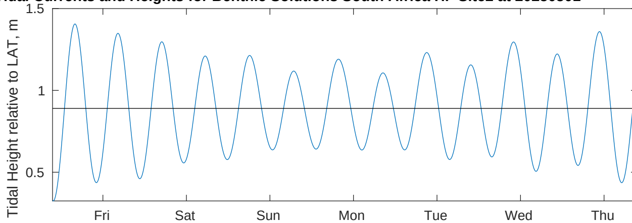
Tidal Currents and Heights for Benthic Solutions South Africa HF Site2 at 20250501
