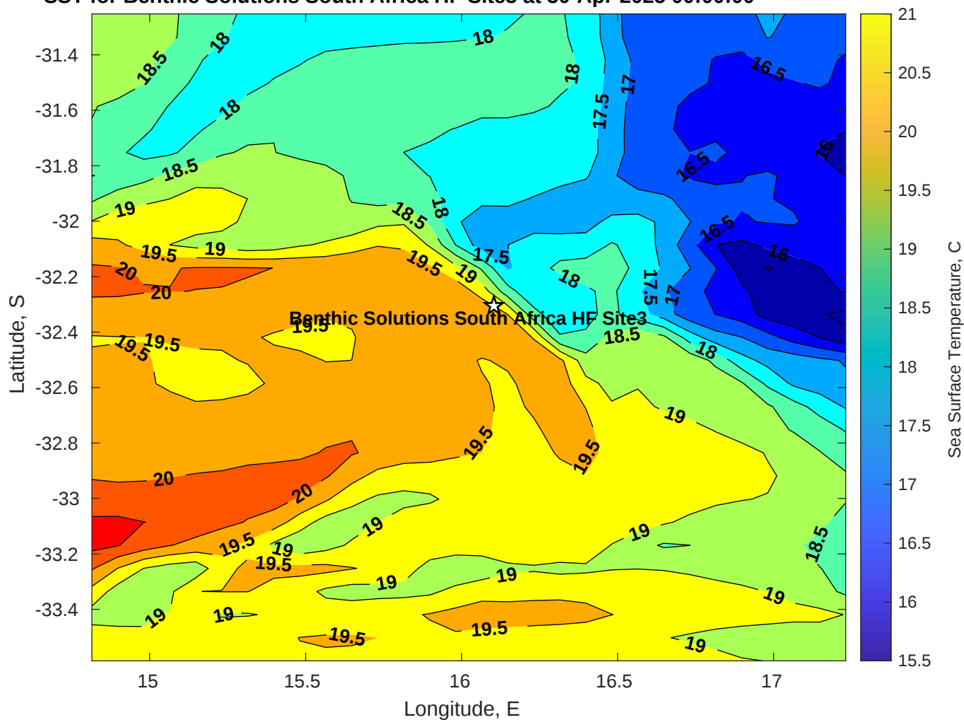
SST for Benthic Solutions South Africa HF Site3 at 30-Apr-2025 00:00:00
