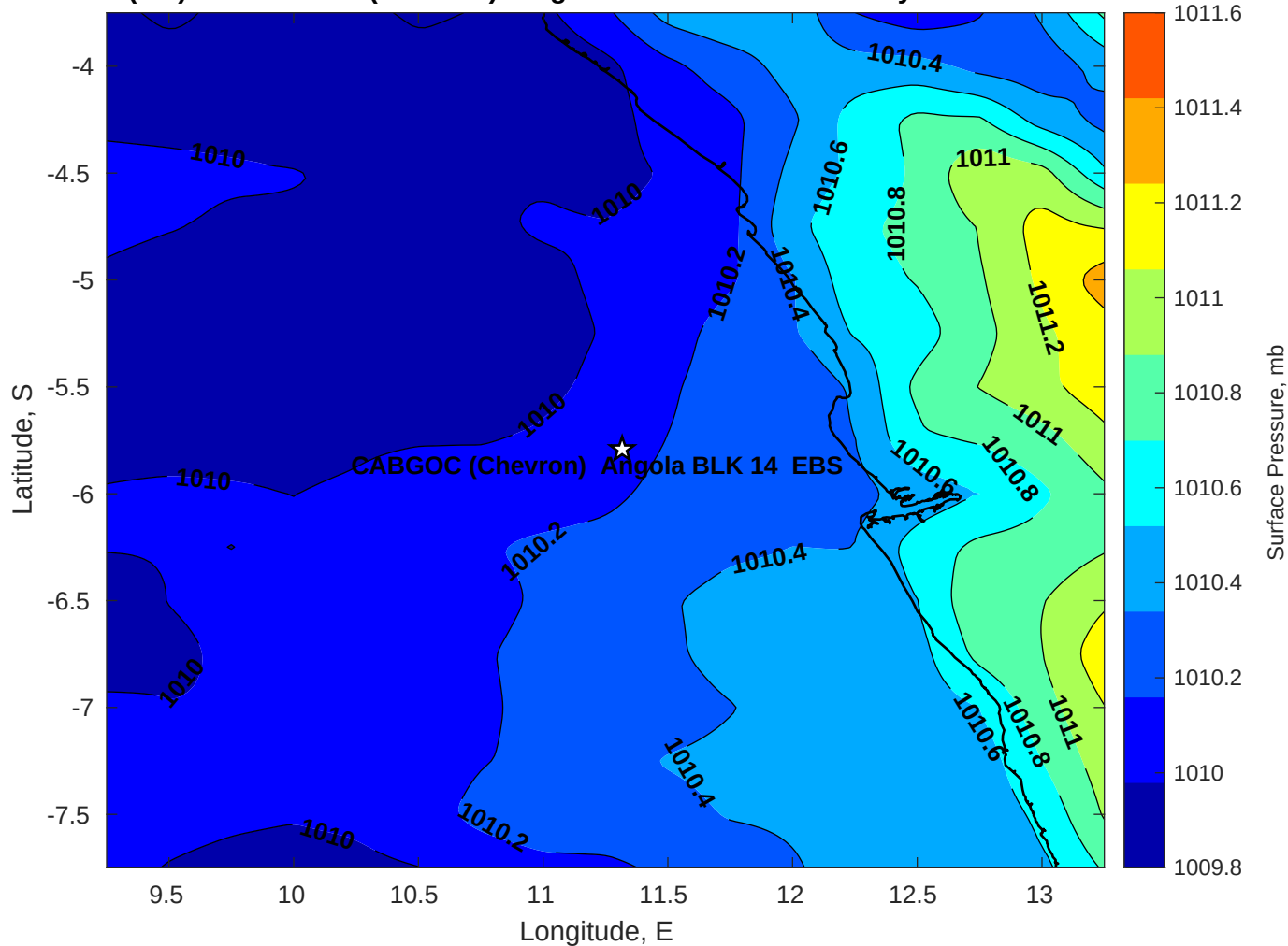
Surface Pressure (mb) for CABGOC (Chevron) Angola BLK 14 EBS at 02-May-2025 00:00:00
