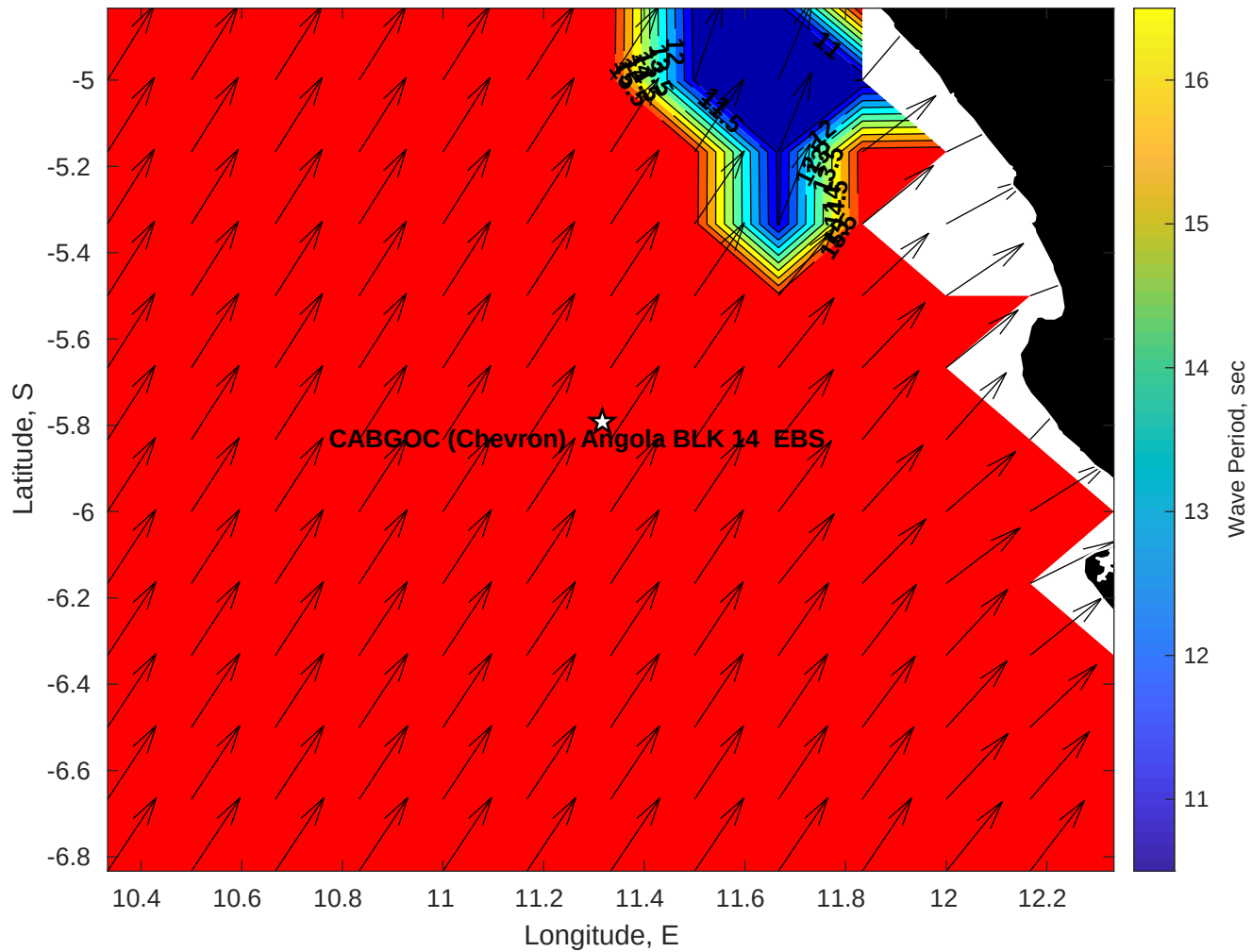
Wave Period (sec) for CABGOC (Chevron) Angola BLK 14 EBS at 01-May-2025 09:00:00
