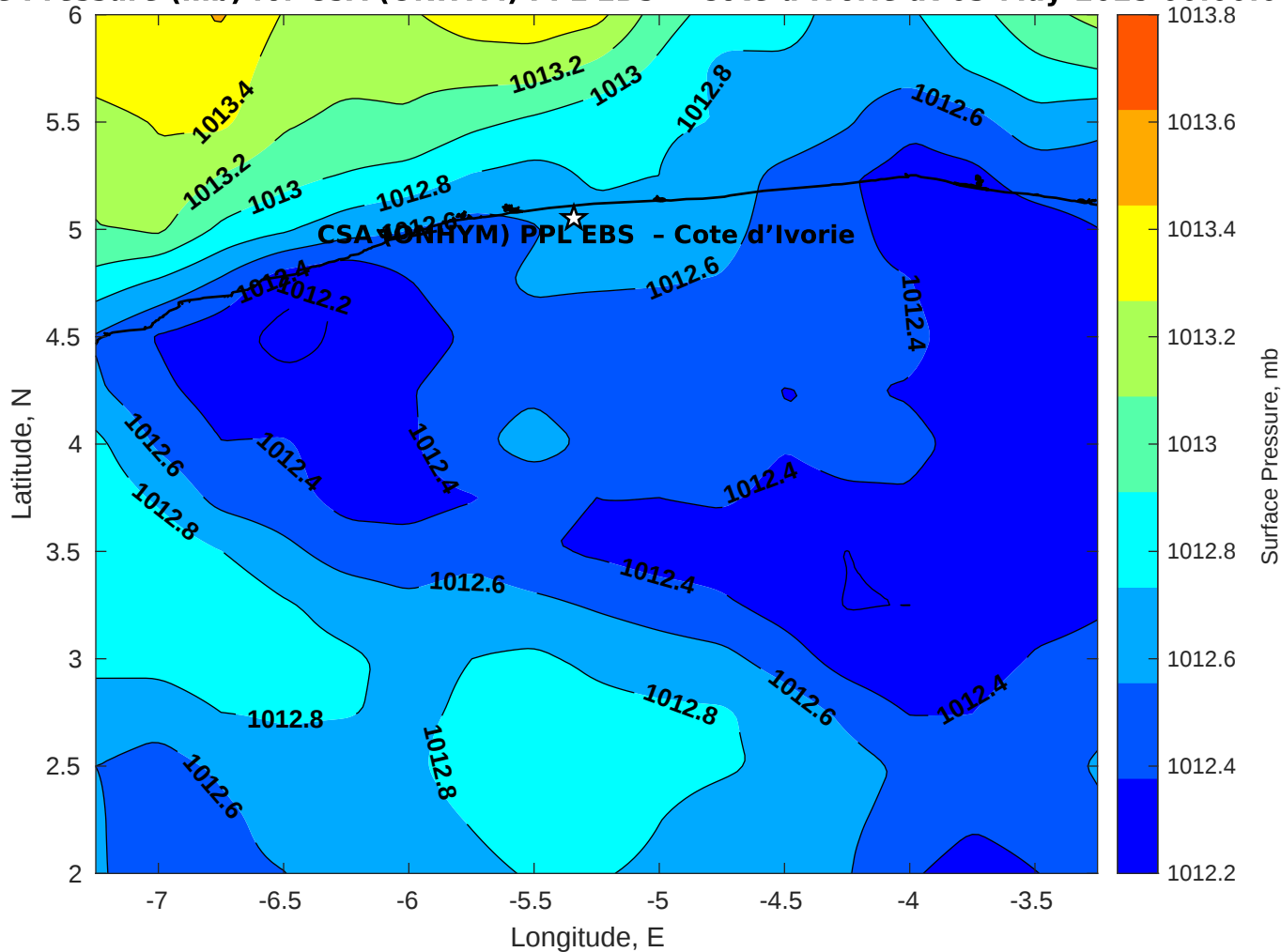
Surface Pressure (mb) for CSA (ONHYM) PPL EBS - Cote d'Ivoire at 03-May-2025 00:00:00
