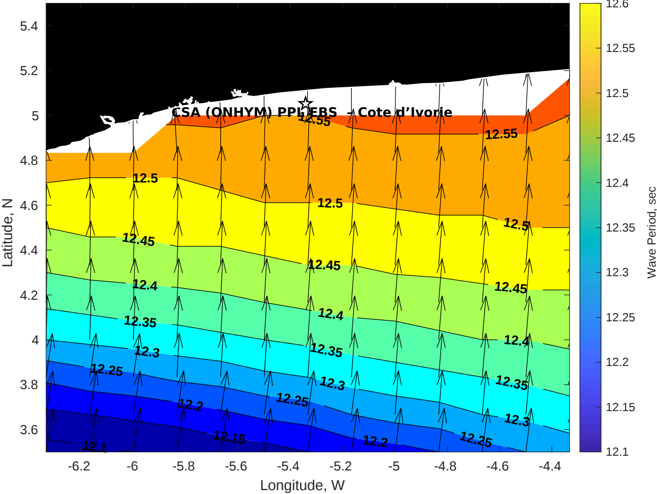
Wave Period (sec) for CSA (ONHYM) PPL EBS - Cote d'Ivoire at 01-May-2025 09:00:00
