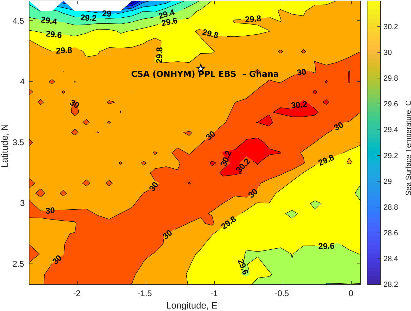
SST for CSA (ONHYM) PPL EBS - Ghana at 30-Apr-2025 00:00:00
