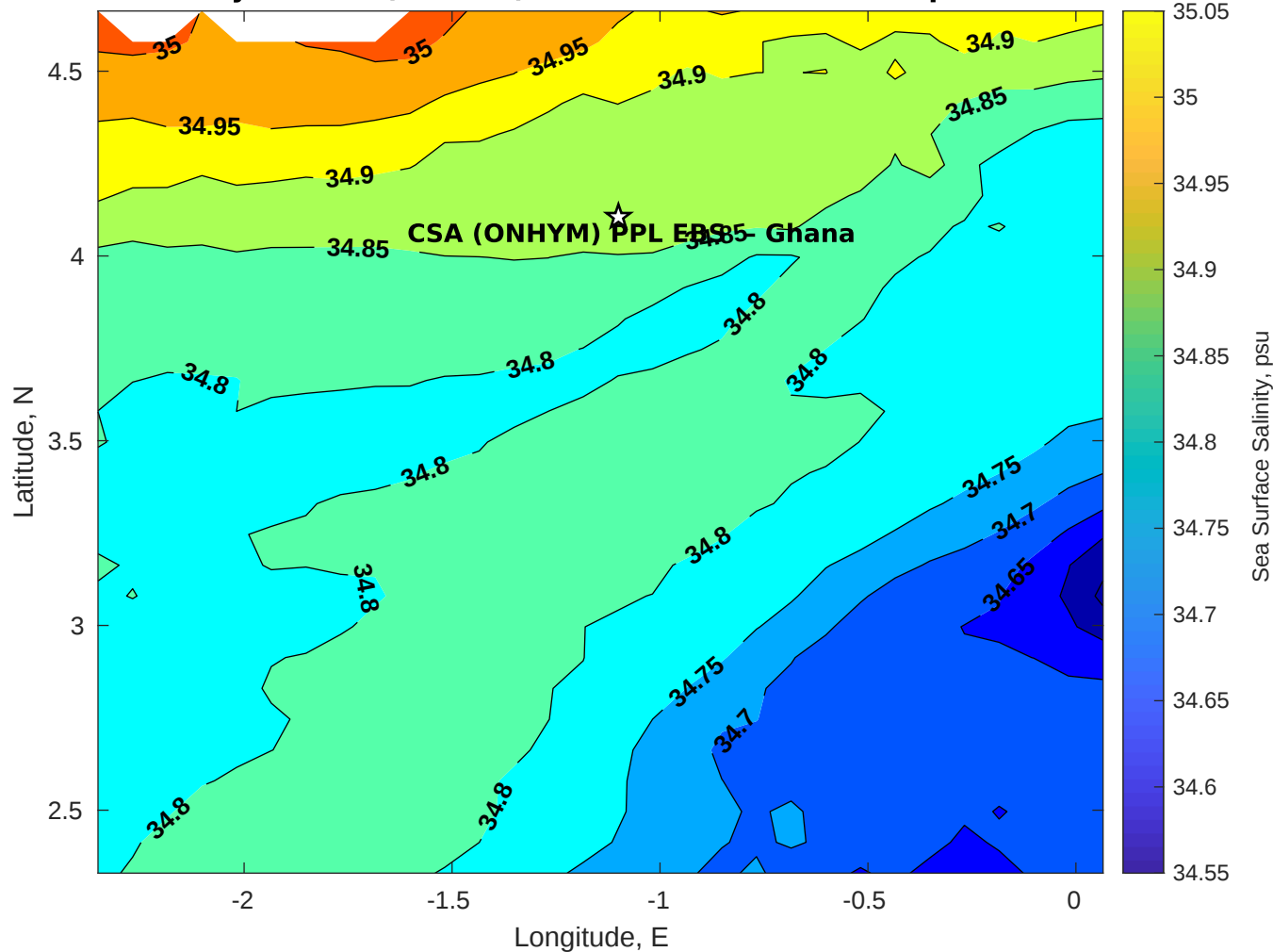
Surface Salinity for CSA (ONHYM) PPL EBS - Ghana at 30-Apr-2025 00:00:00
