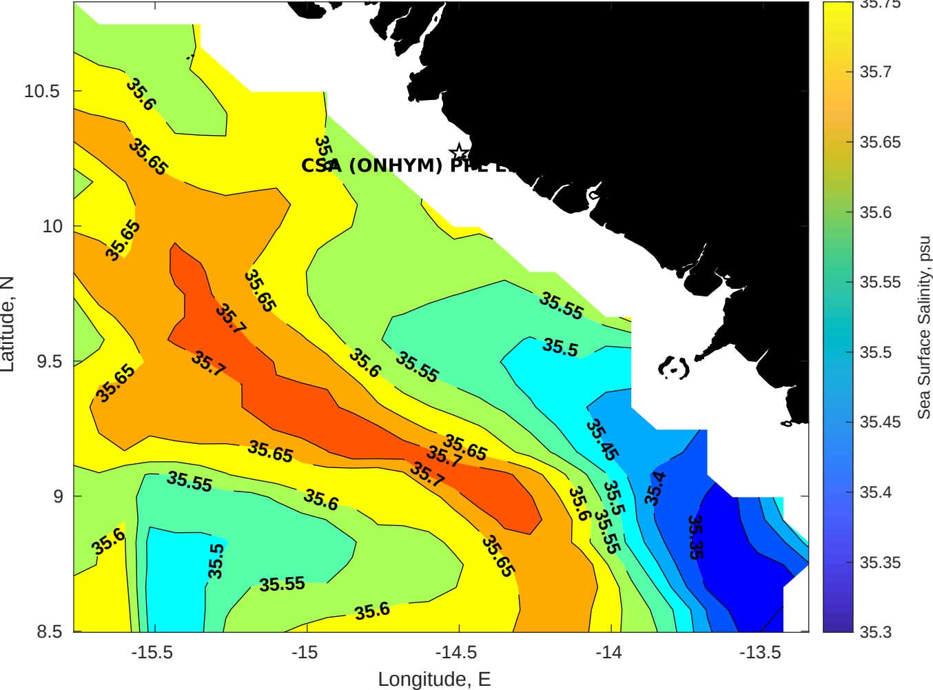
Surface Salinity for CSA (ONHYM) PPL EBS - Guinea at 30-Apr-2025 00:00:00
