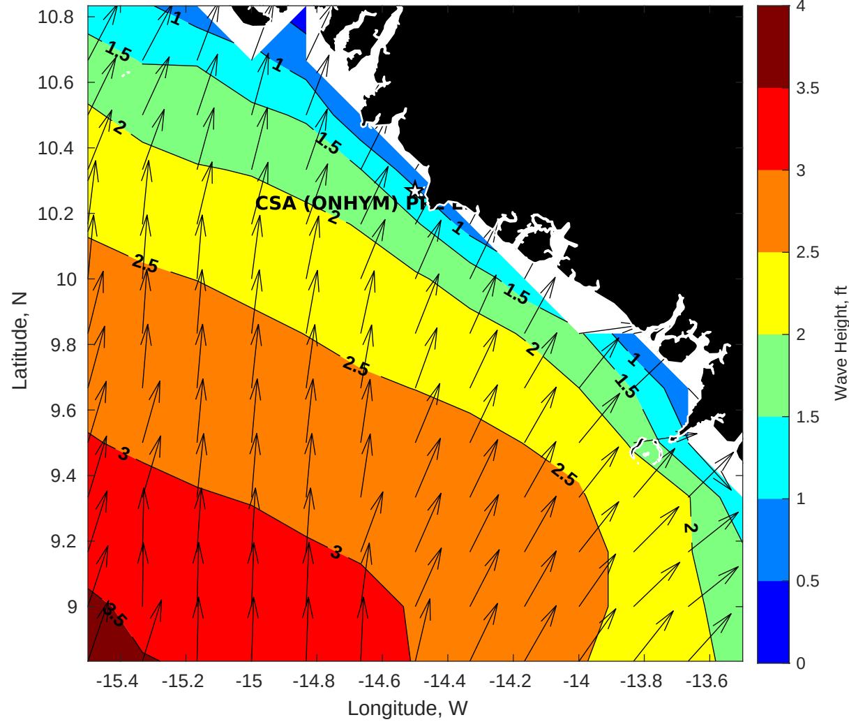
Wave Height (ft) for CSA (ONHYM) PPL EBS - Guinea at 01-May-2025 09:00:00
