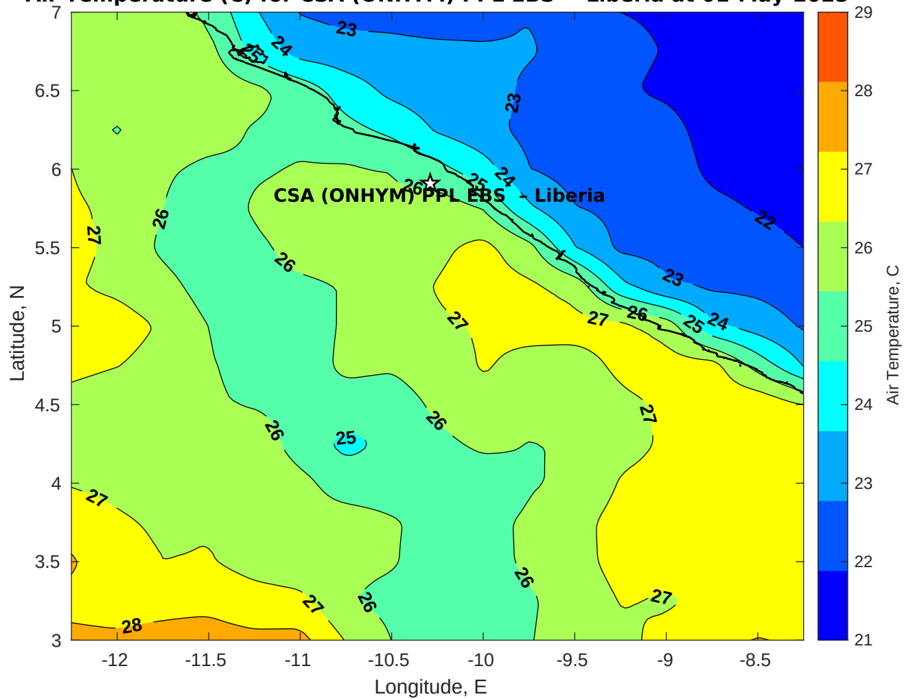
Air Temperature (C) for CSA (ONHYM) PPL EBS - Liberia at 01-May-2025
