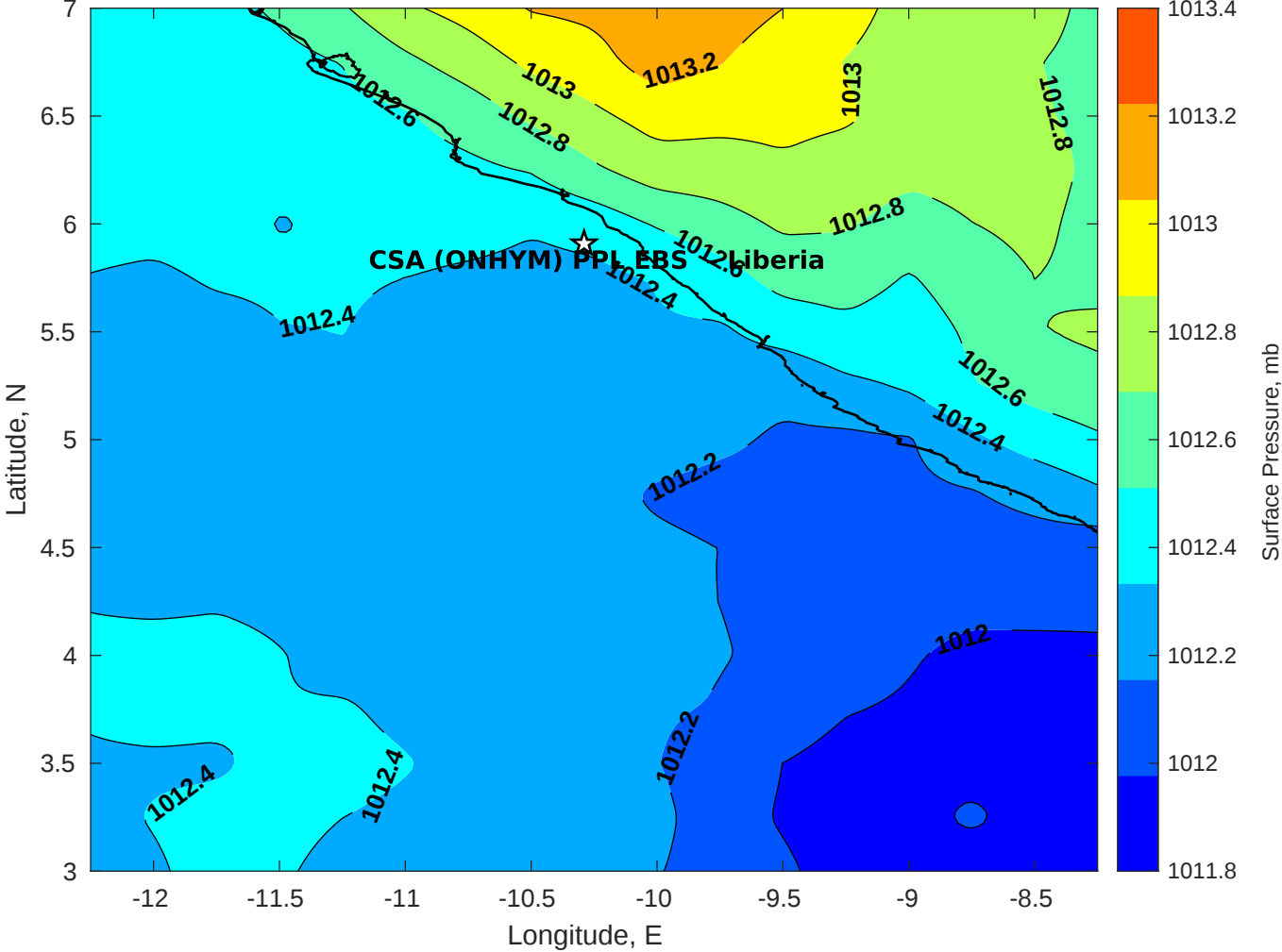
Surface Pressure (mb) for CSA (ONHYM) PPL EBS - Liberia at 02-May-2025 00:00:00
