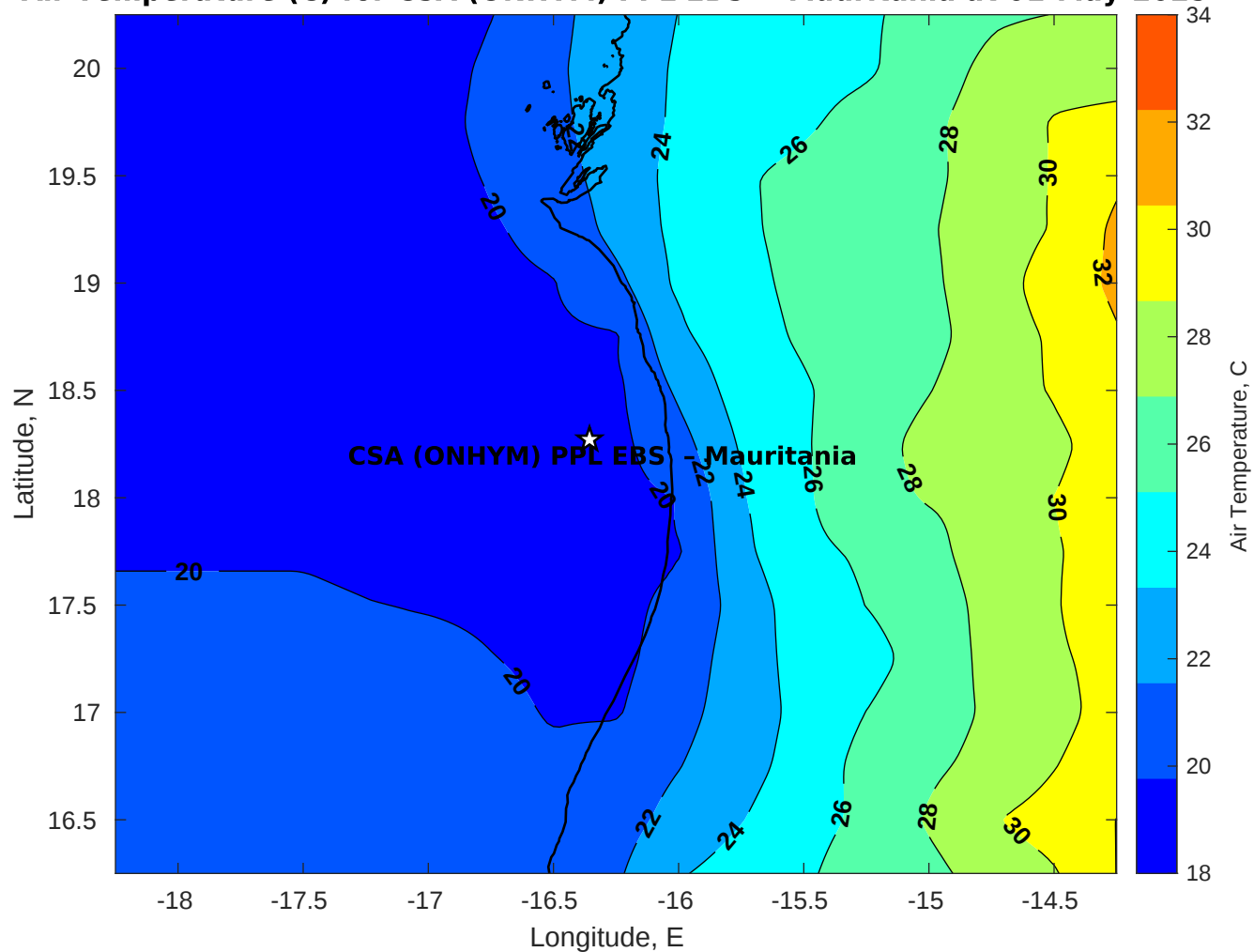
Air Temperature (C) for CSA (ONHYM) PPL EBS - Mauritania at 01-May-2025
