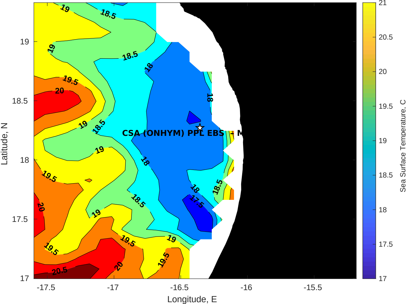
SST for CSA (ONHYM) PPL EBS - Mauritania at 30-Apr-2025 00:00:00
