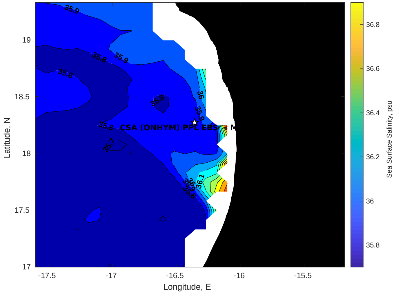
Surface Salinity for CSA (ONHYM) PPL EBS - Mauritania at 30-Apr-2025 00:00:00
