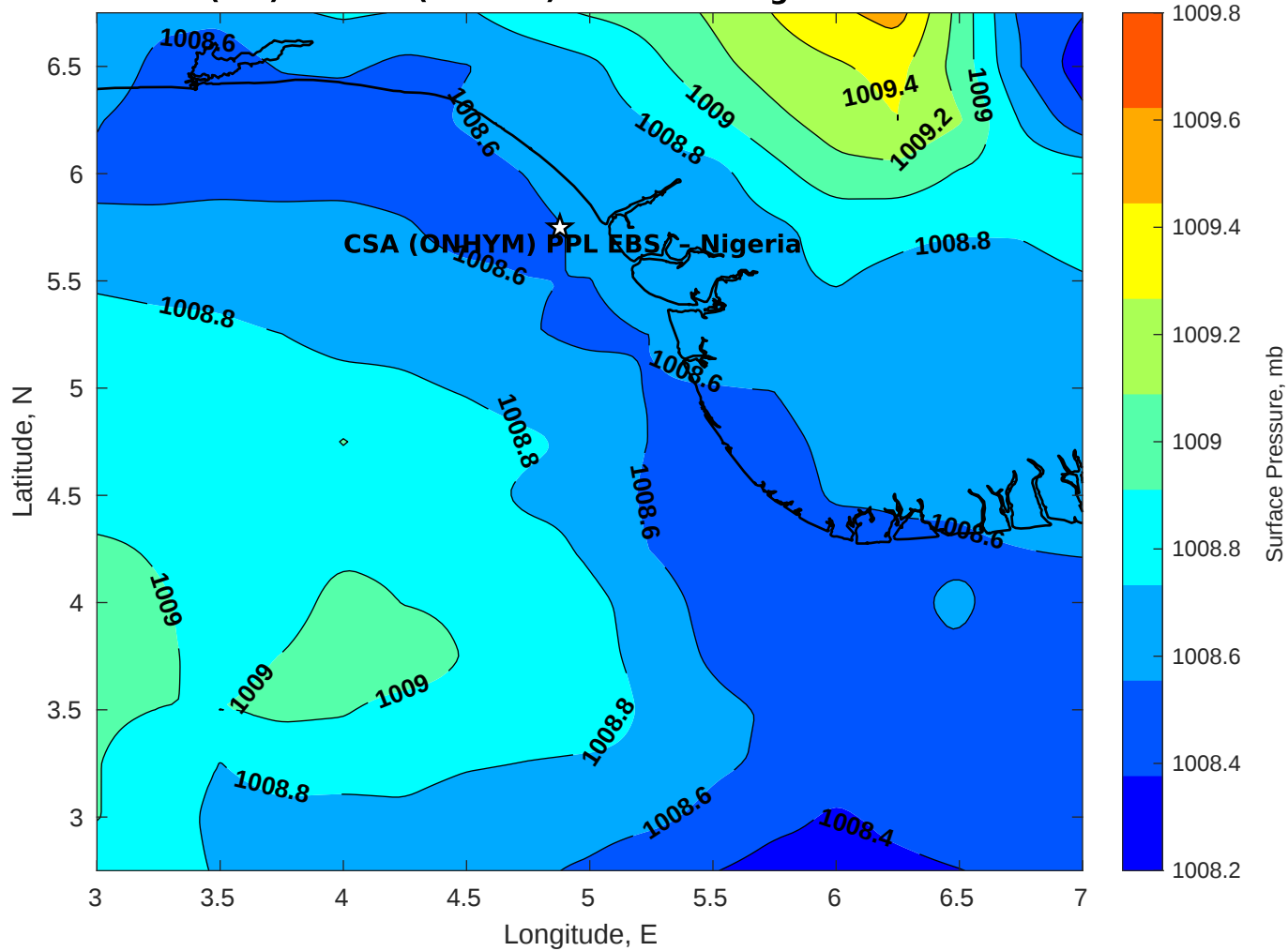
Surface Pressure (mb) for CSA (ONHYM) PPL EBS - Nigeria at 15-Nov-2030 00:00:00
