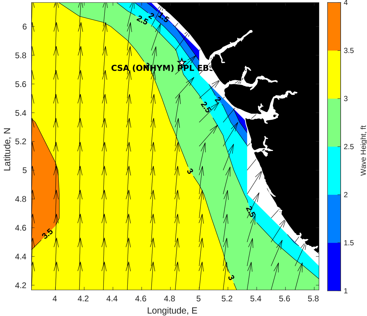
Wave Height (ft) for CSA (ONHYM) PPL EBS - Nigeria at 01-May-2025 09:00:00
