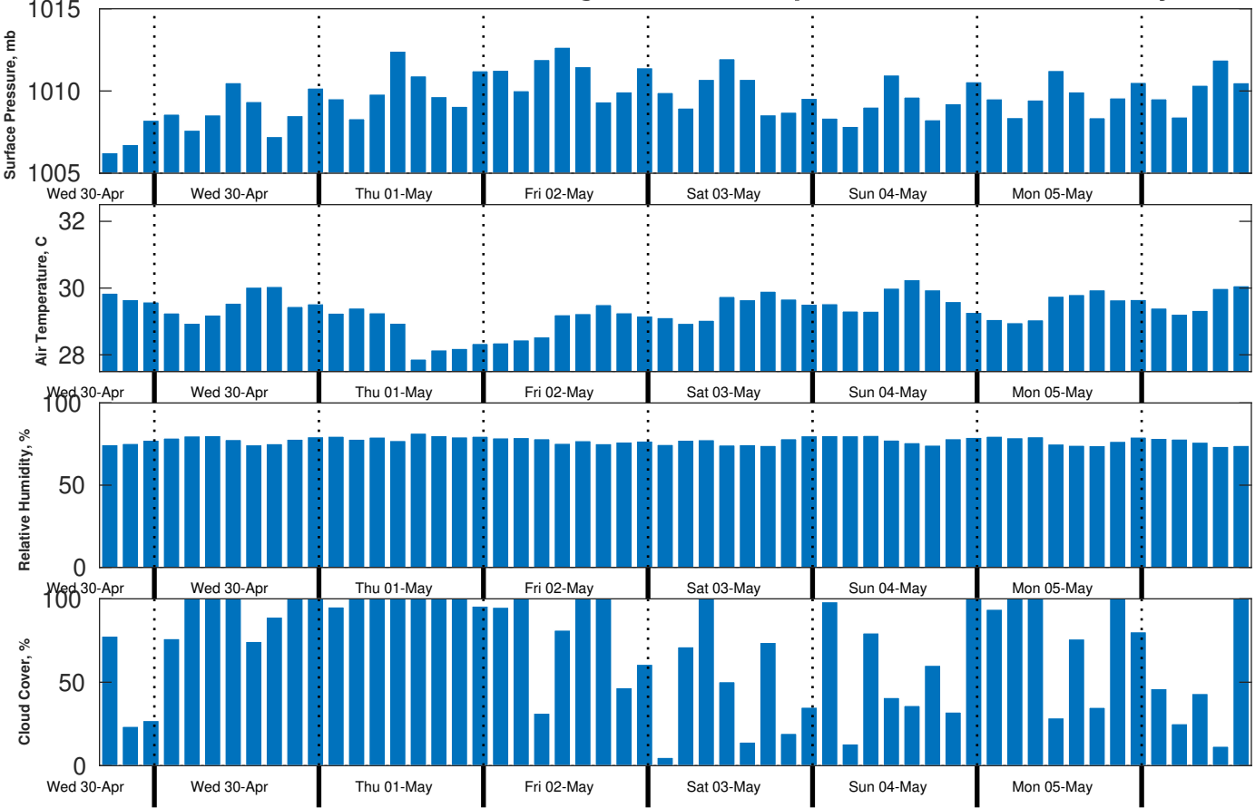
Met Forecast for CSA (ONHYM) PPL EBS - Nigeria from 30-Apr-2025 12:00:00 to 07-May-2025 12:00:00
