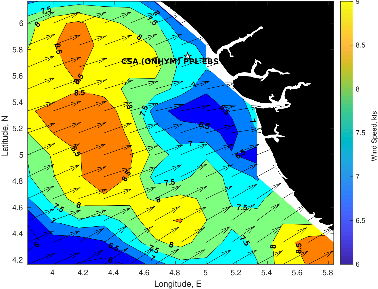
Winds (kts) for CSA (ONHYM) PPL EBS - Nigeria at 01-May-2025 09:00:00
