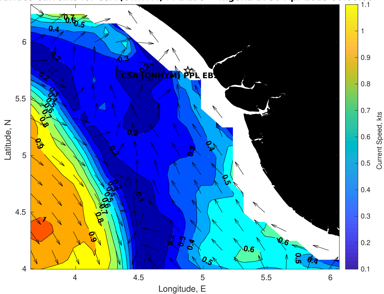
Surface Currents for CSA (ONHYM) PPL EBS - Nigeria at 30-Apr-2025 00:00:00
