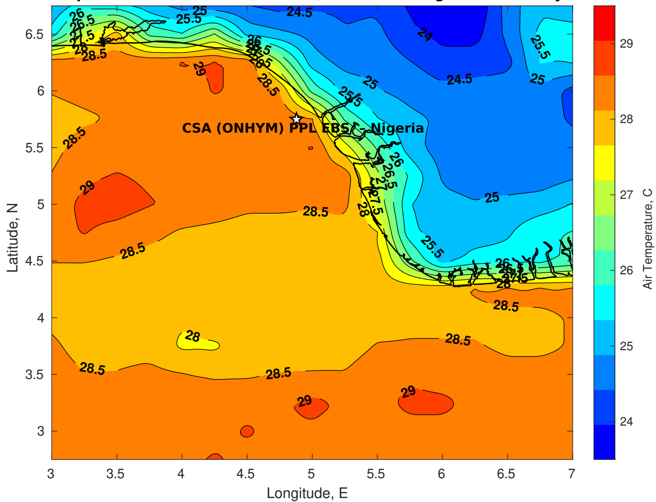
Air Temperature (C) for CSA (ONHYM) PPL EBS - Nigeria at 01-May-2025
