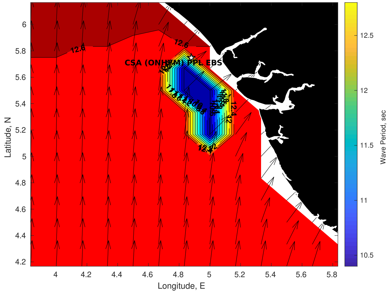
Wave Period (sec) for CSA (ONHYM) PPL EBS - Nigeria at 01-May-2025 09:00:00
