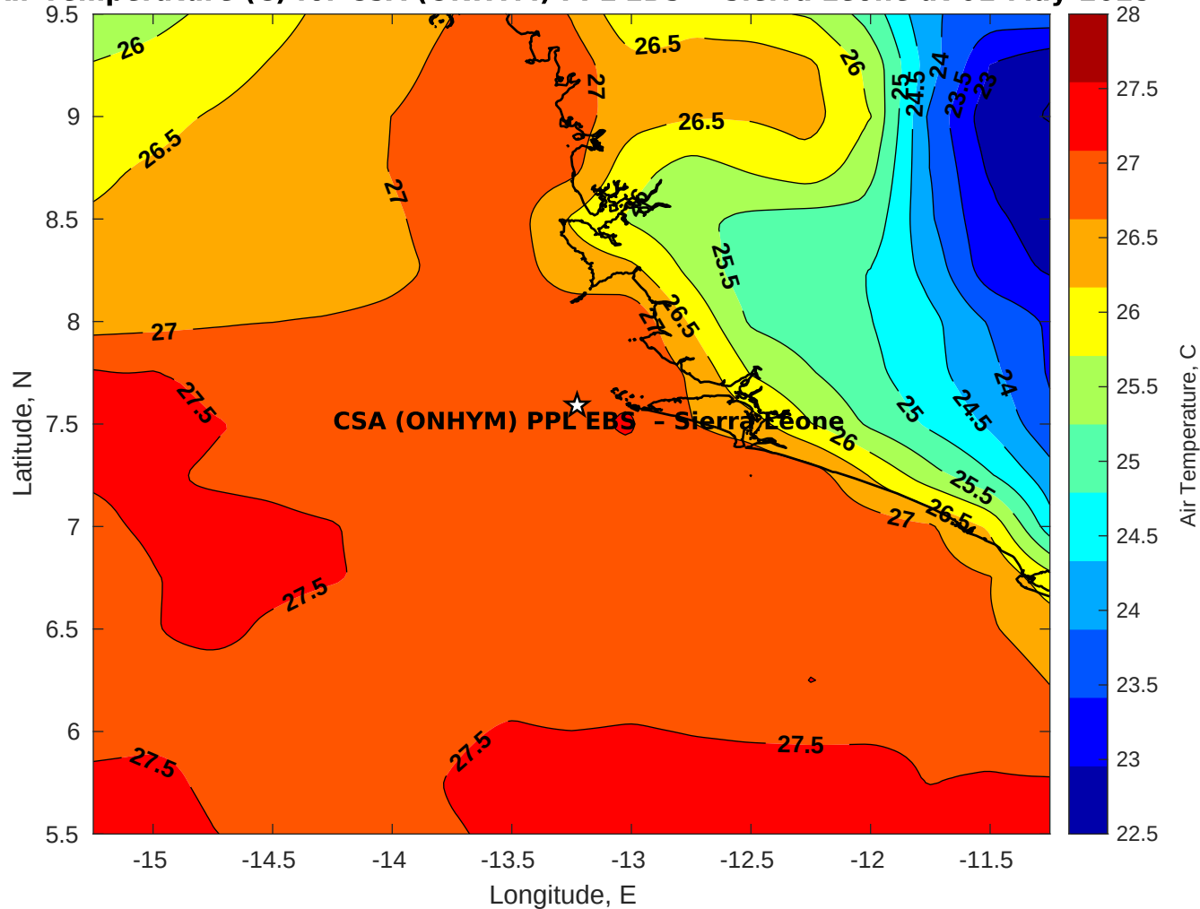
Air Temperature (C) for CSA (ONHYM) PPL EBS - Sierra Leone at 01-May-2025
